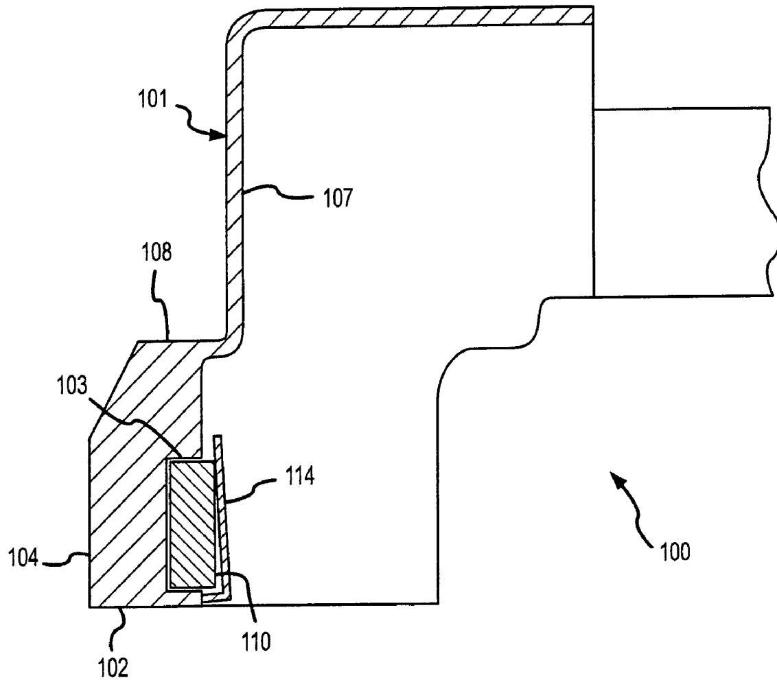
SECTION FIG. 4
