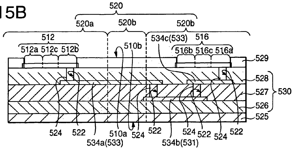
SEMICONDUCTOR CHIP ACCORDING TO FIFTH EMBODIMENT
