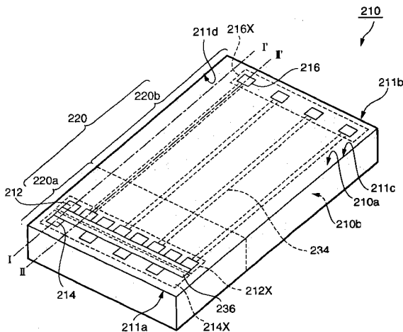
EXAMPLE OF PACKAGING OF SEMICONDUCTOR CHIPS ACCORDING TO SECOND EMBODIMENT
