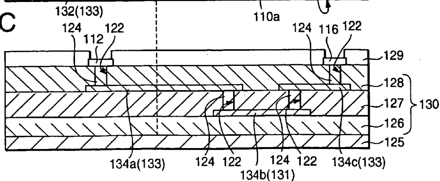
SEMICONDUCTOR CHIP ACCORDING TO FIRST EMBODIMENT
