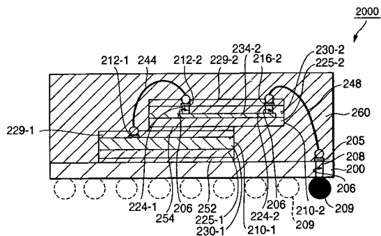
EXAMPLE OF PACKAGING OF SEMICONDUCTOR CHIPS ACCORDING TO SECOND EMBODIMENT
