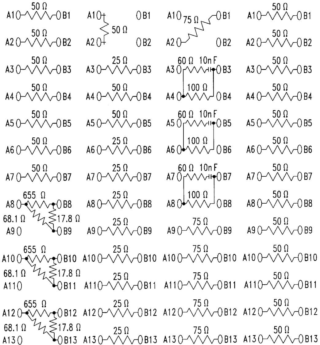
FIG. 3 PRIOR ART
