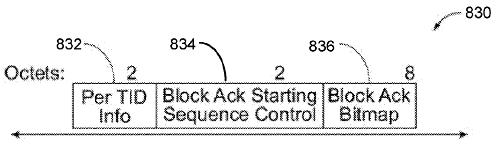
Block Acknowledgment Information Field
