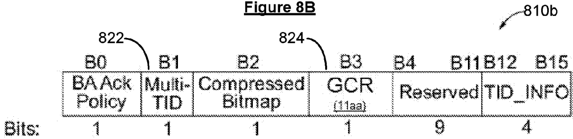
Block Acknowledgment Control Field (11aa)
