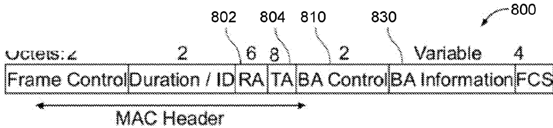
Block Acknowledgment Frame
