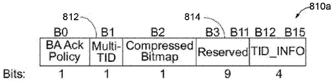
Block Acknowledgment Control Field
