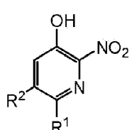
Structure 6b
