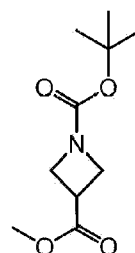
Structure 12
