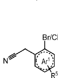
Structure 8
