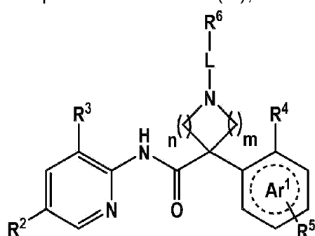
Formula (III)
