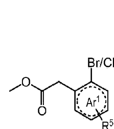
Structure 9
