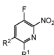
Structure 7b
