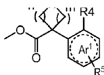
Structure 5
