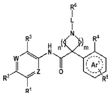
Formel (I)
