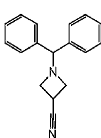
Structure 10
