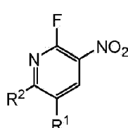
Structure 7a
