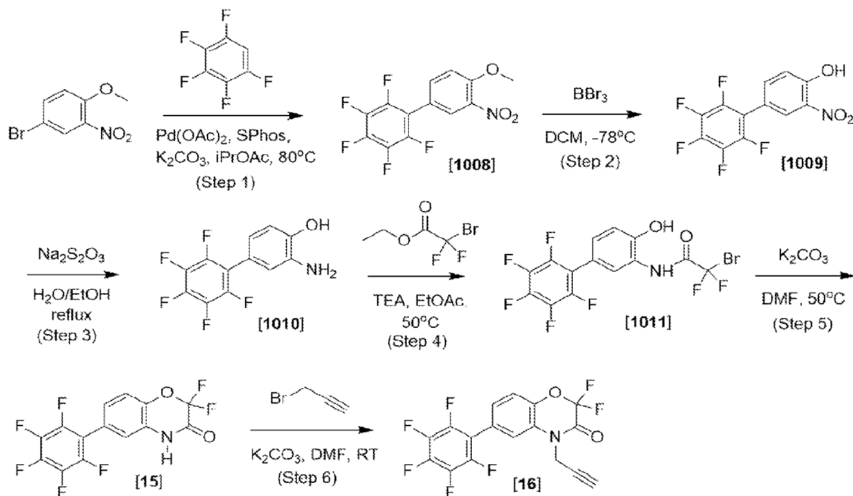
Scheme 7
