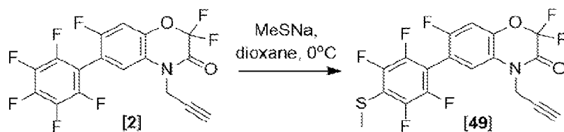
Scheme 26
