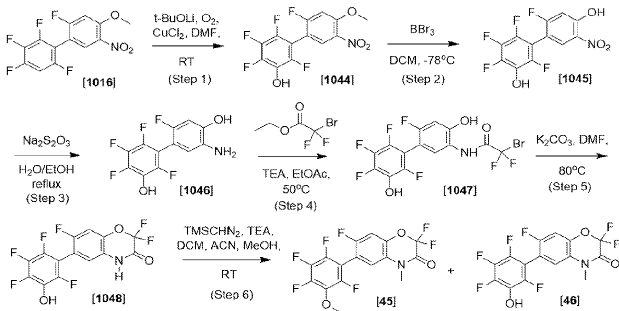
Scheme 23
