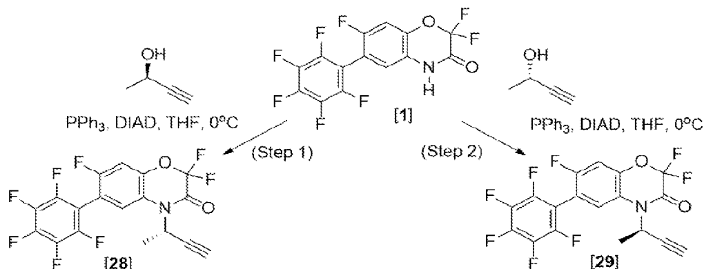
Scheme 11
