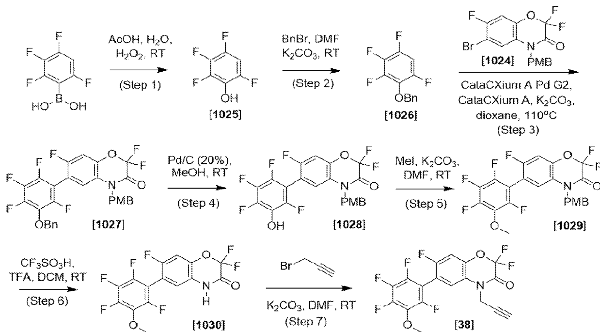
Scheme 18
