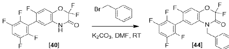
Scheme 22
