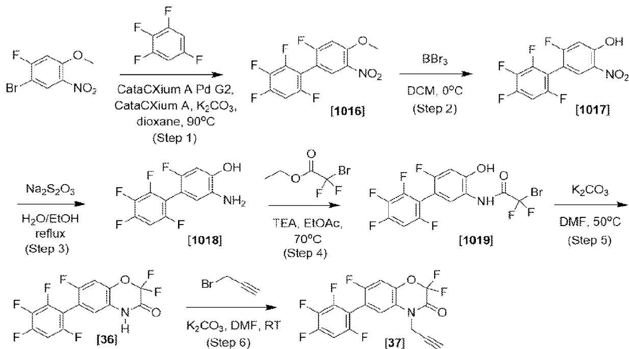
Scheme 16
