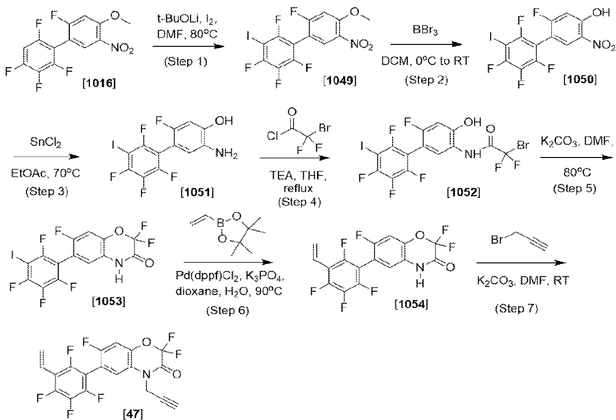
Scheme 24
