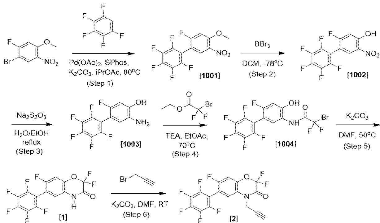
Scheme 3
