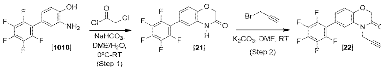
Scheme 8
