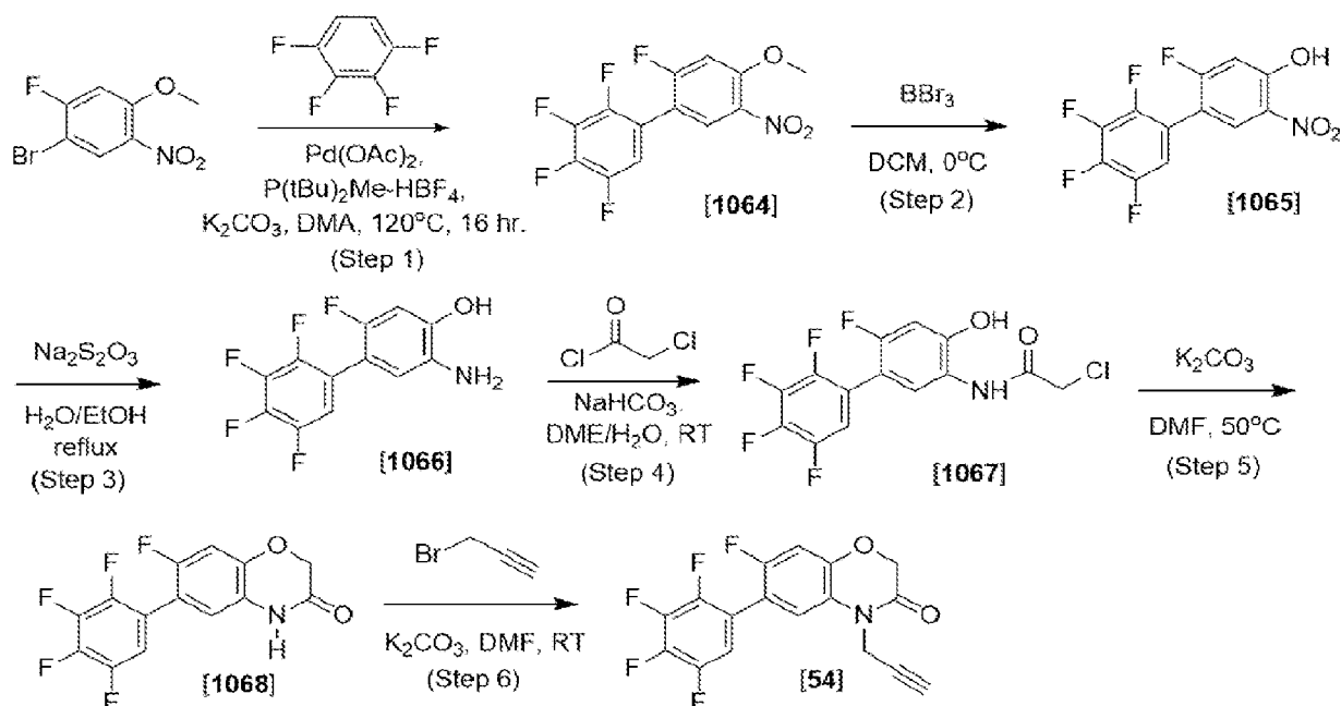
Scheme 31
