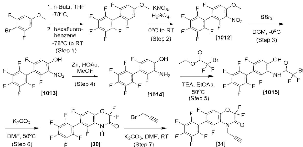
Scheme 12
