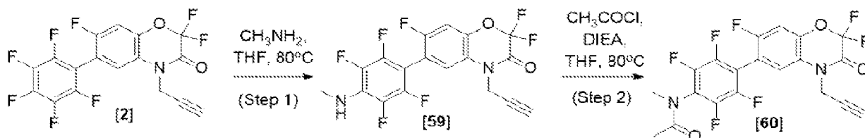
Scheme 35
