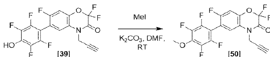
Scheme 27
