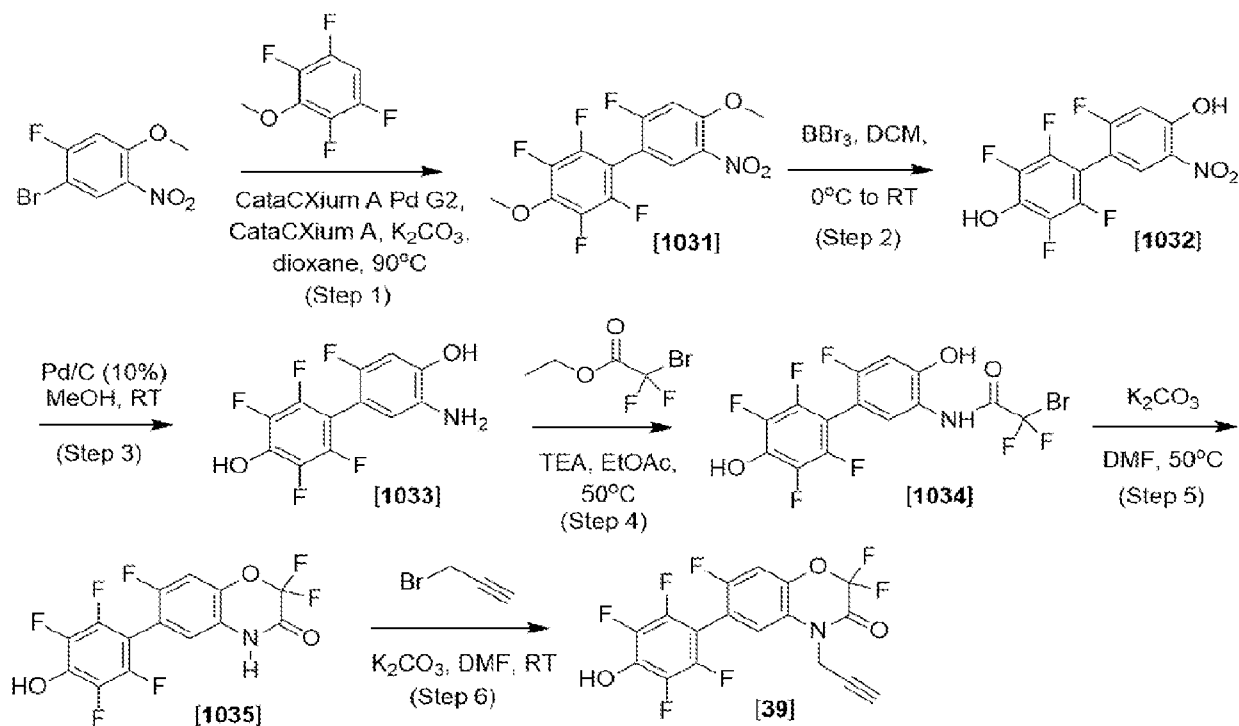
Scheme 19
