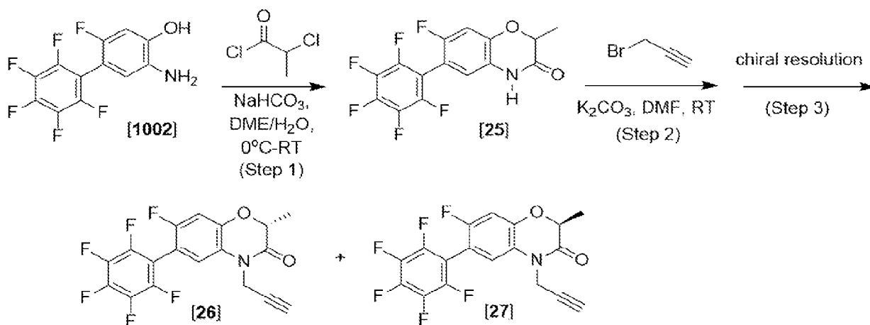
Scheme 10
