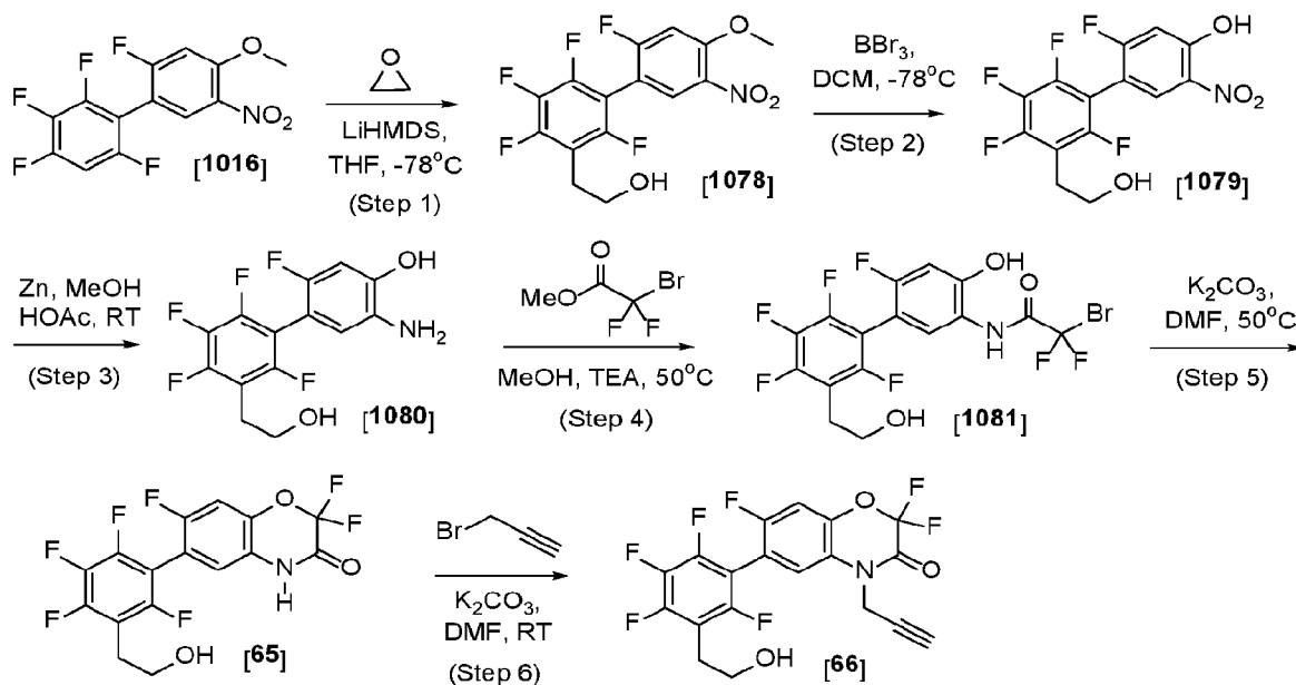
Scheme 39
