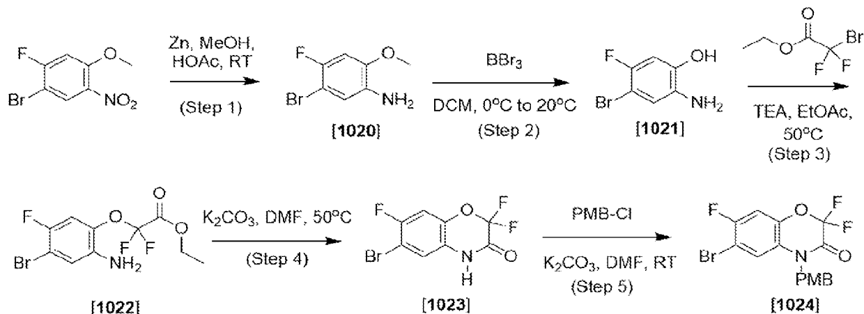
Scheme 17
