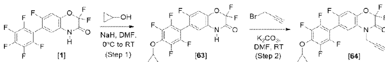
Scheme 38
