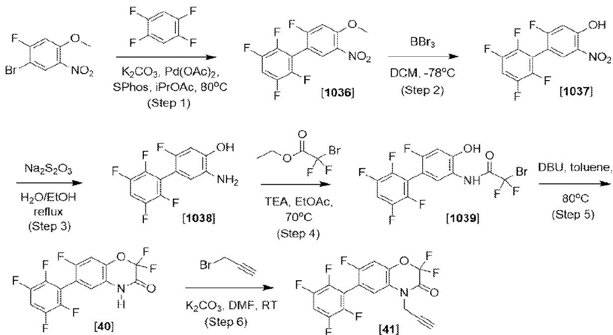
Scheme 20
