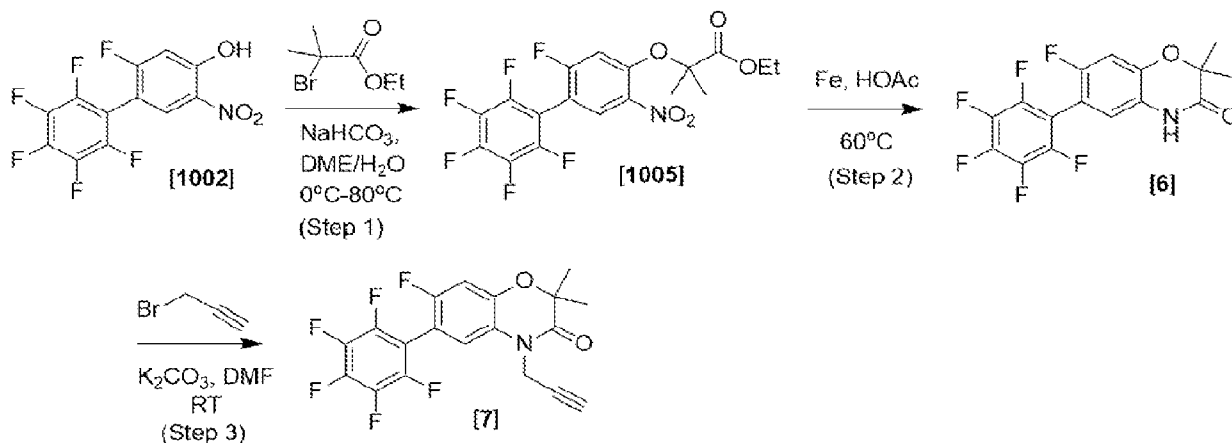
Scheme 5
