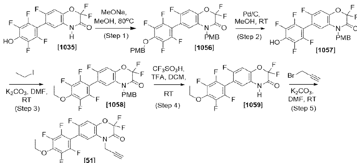
Scheme 28
