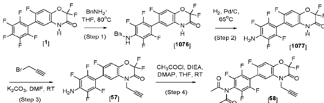
Scheme 34
