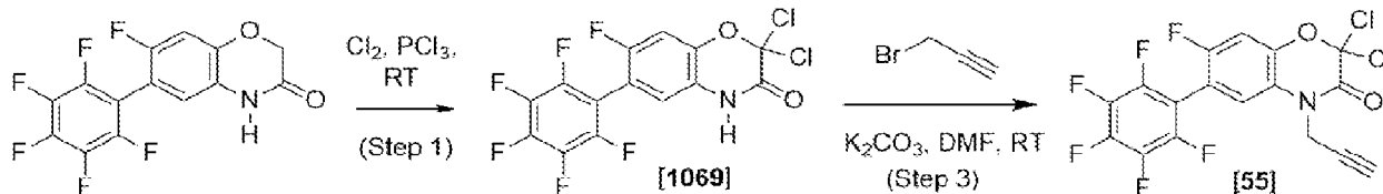
Scheme 32
