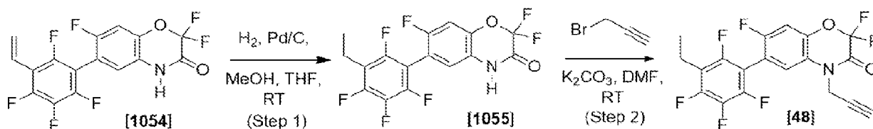
Scheme 25
