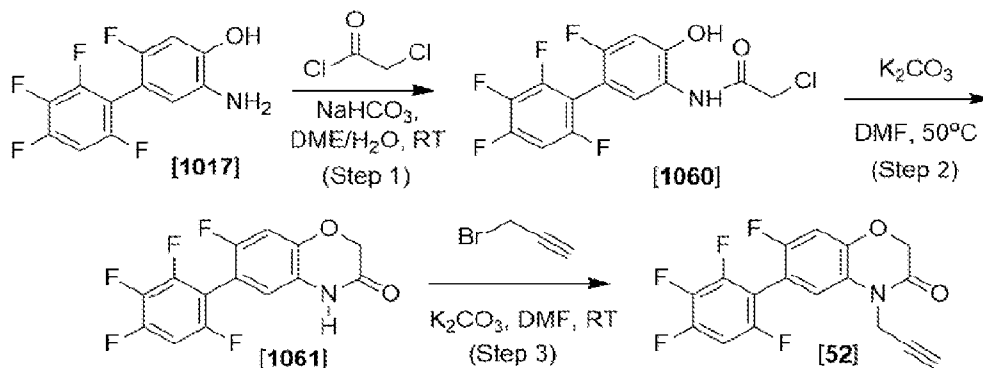
Scheme 29
