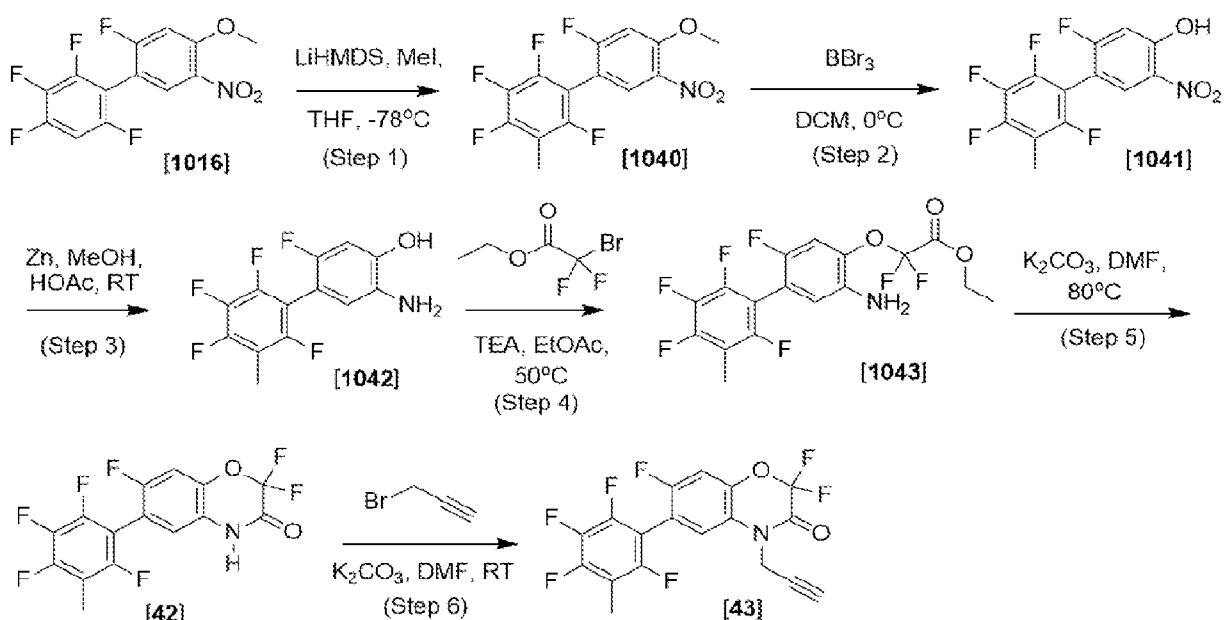
Scheme 21
