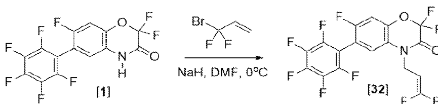
Scheme 13
