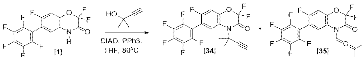
Scheme 15
