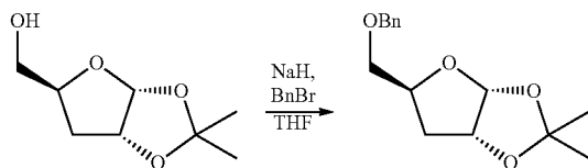
(3 \alpha R,5S,6 \alpha R)-5-(benzyloxymethyl)-2,2-dimethyl-tetrahydrofuro[2,3-d][1,3]dioxole
