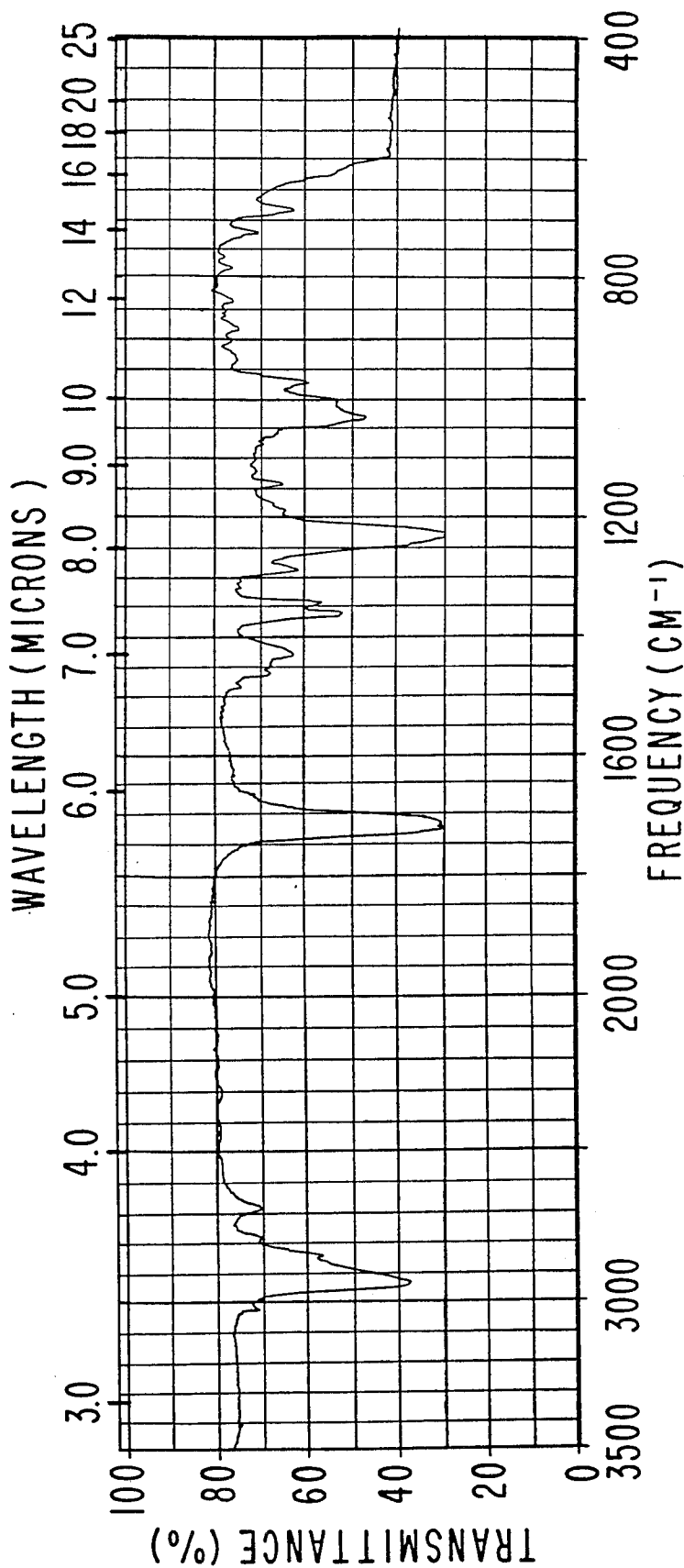
IR SPECTRUM FOR EXAMPLE VIII.
