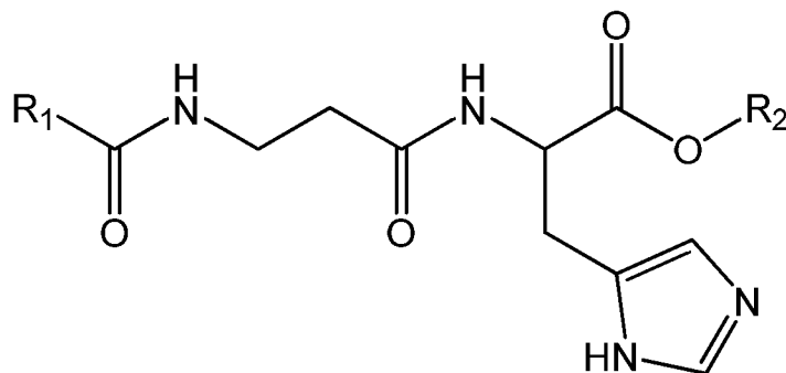
(Formula III) Carnosine Derivatives
