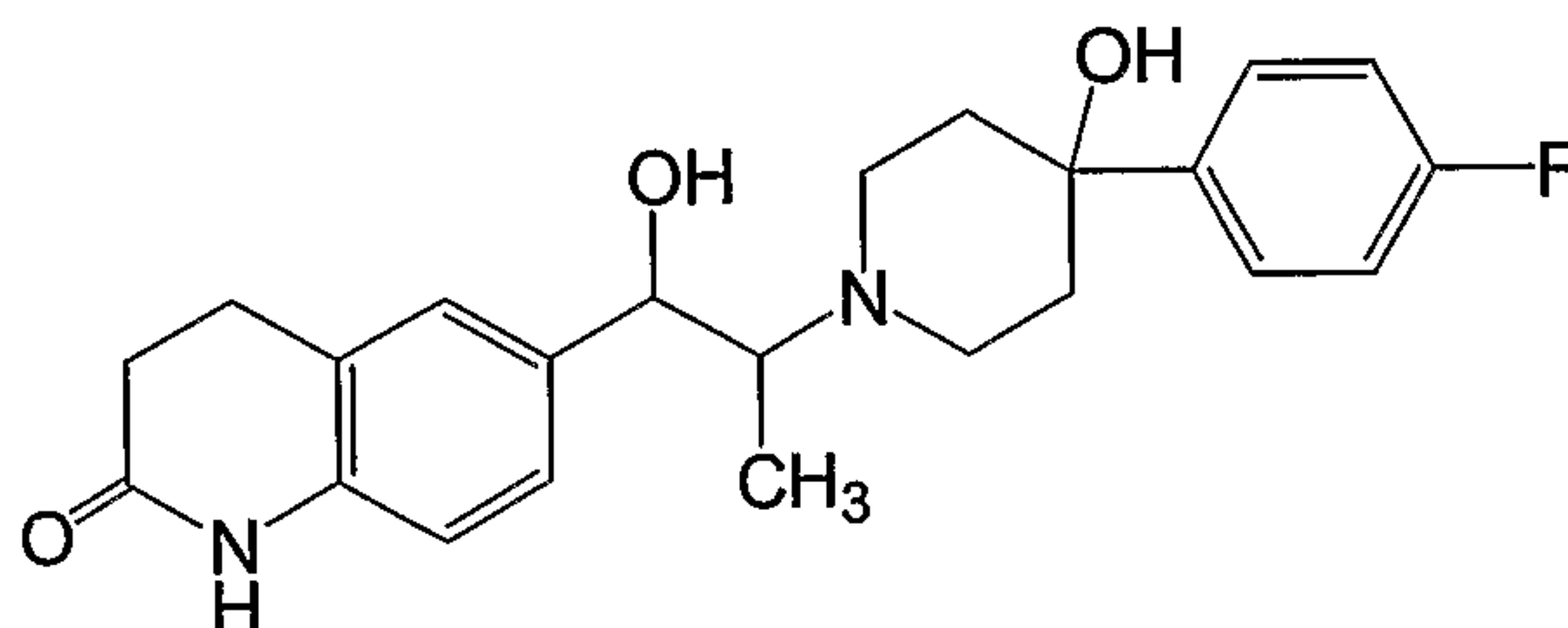
Compound A
