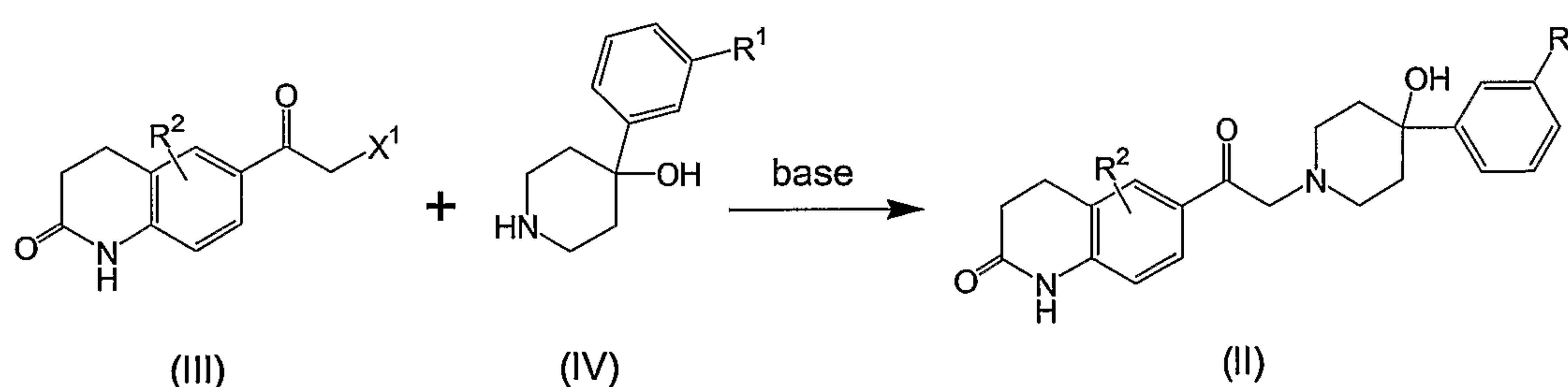
Scheme II
