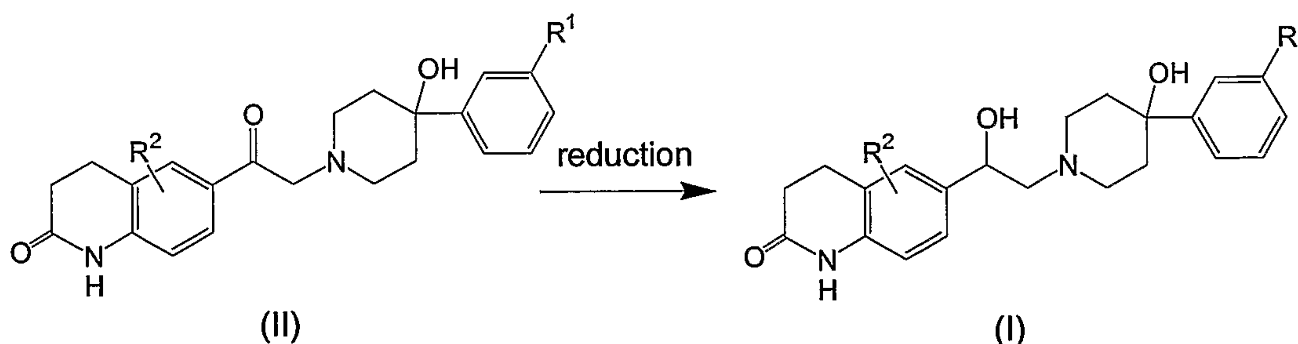
Scheme I
