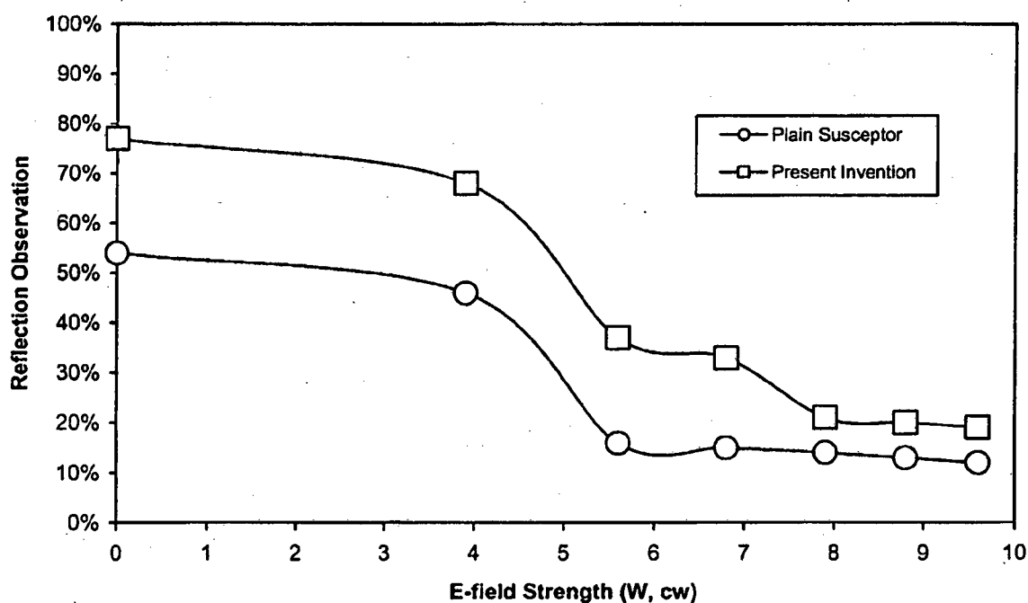
Reflection Characteristics
