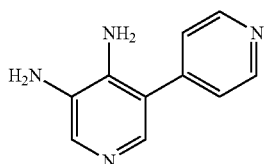
3,4'-bipyridine-4,5-diamine (LII)
