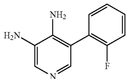
5-(2-fluorophenyl)pyridine-3,4-diamine (LI)
