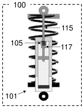
Full rebound FIG. 3A
