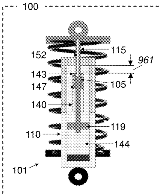
Design FIG. 19A
