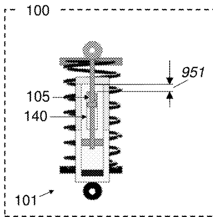
Design FIG. 17A
