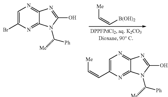
(S,Z)-1-(1-phenylethyl)-6-(prop-1-enyl)-1H-imidazo[4,5-b]pyrazin-2-ol
