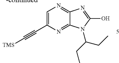
1-(pentan-3-yl)-6-((trimethylsilyl)ethynyl)-1H-imidazo[4,5-b]pyrazin-2-ol
