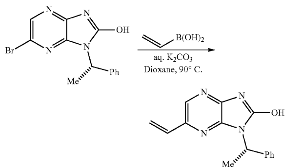
(S)-1-(1-phenylethyl)-6-vinyl-1H-imidazo[4,5-b]pyrazin-2-ol
