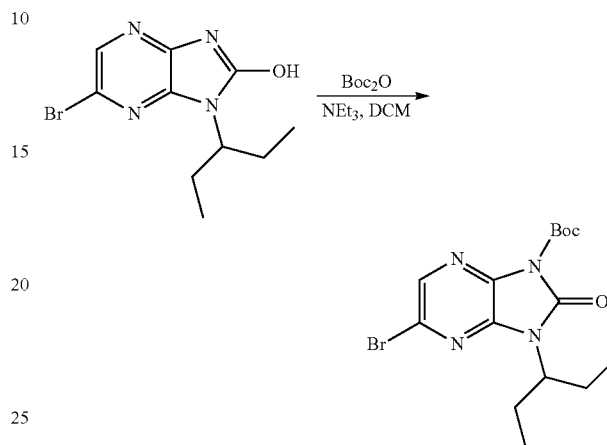
tert-butyl 5-bromo-2-oxo-3-(pentan-3-yl)-2,3-dihydroimidazo[4,5-b]pyrazine-1-carboxylate
