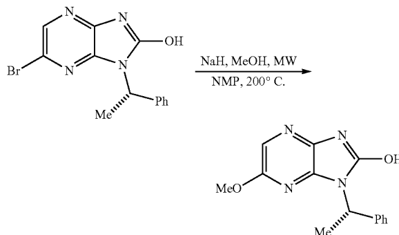
(S)-6-methoxy-1-(1-phenylethyl)-1H-imidazo[4,5-b]pyrazin-2-ol
