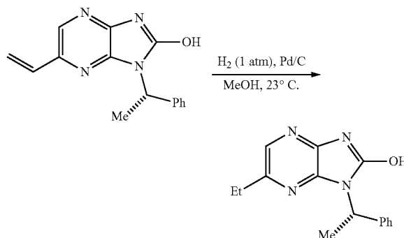
(S)-1-(1-phenylethyl)-6-ethyl-1H-imidazo[4,5-b]pyrazin-2-ol
