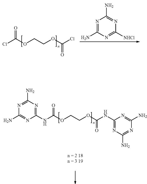
Scheme 8. Preparation of bismelamine carbamates
