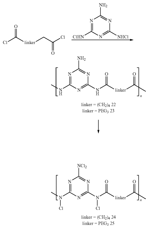
Scheme 9. Preparation of linear polymers bearing melamine groups
