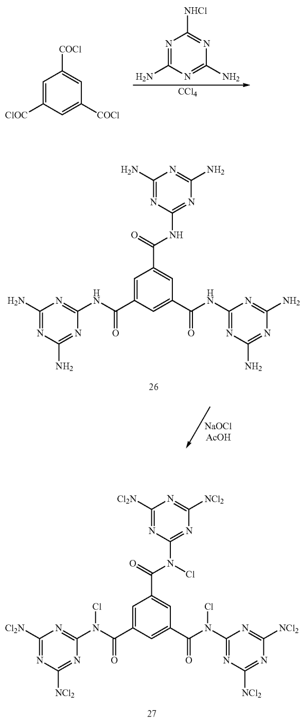
Scheme 10. Preparation of tris-melamineamide
