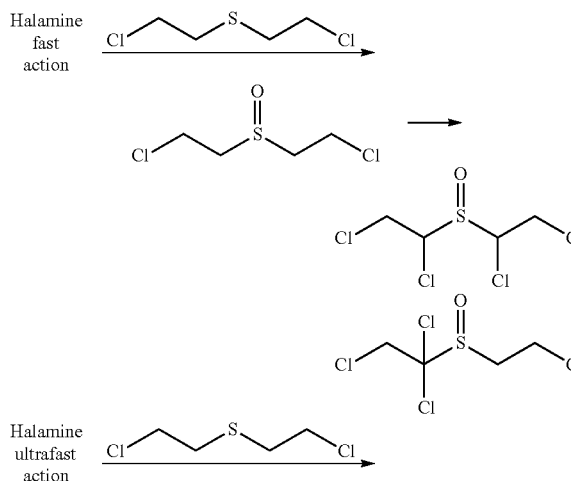
Scheme 13. Proposed mechanism leading to multichlorinated products
