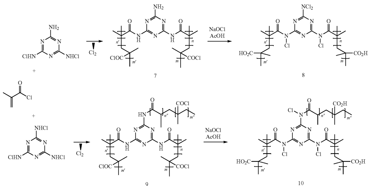
Scheme 4. Preparation of cross-linked melamine-methacrylate polymer
