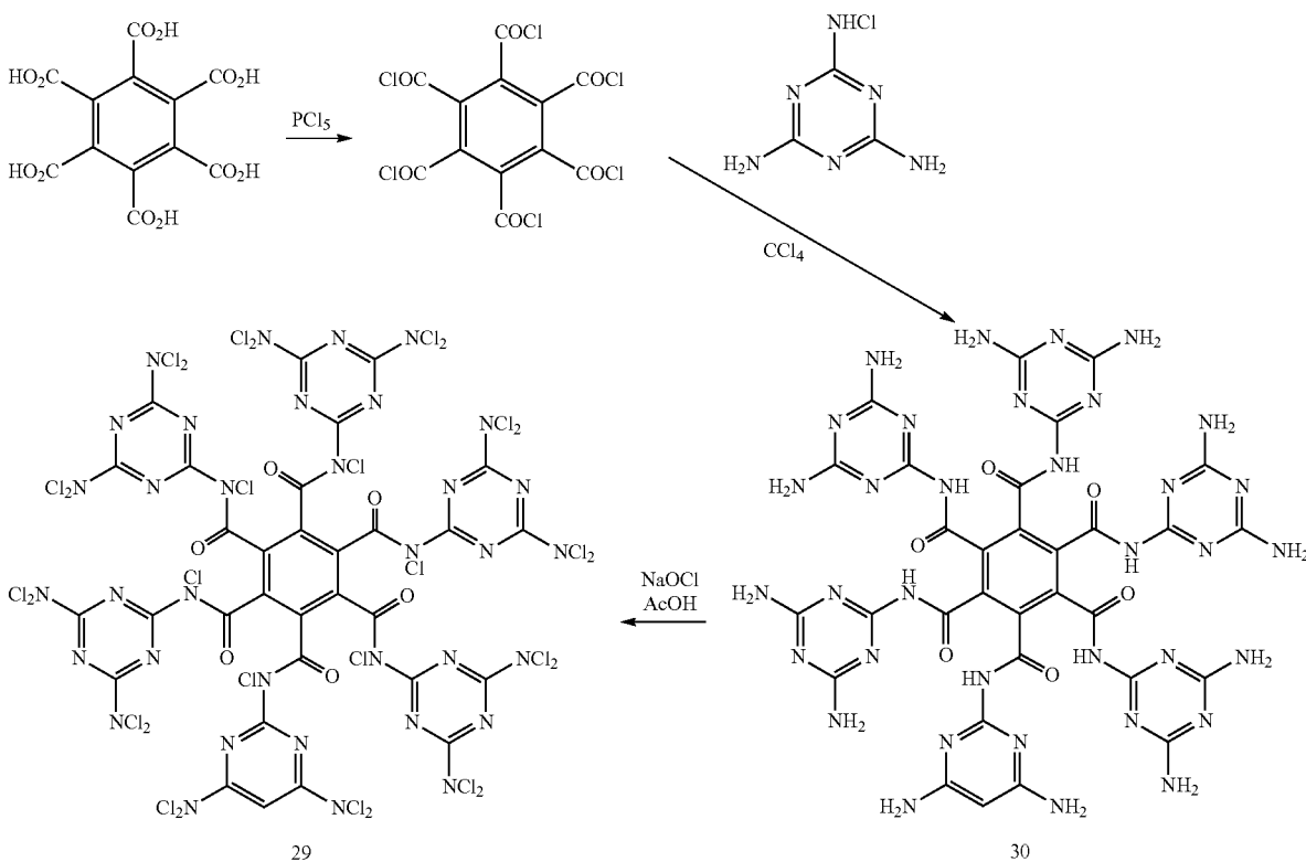
Scheme 12. Preparation of hexakis-melamineamide
