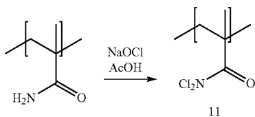
Scheme 5. Preparation of chlorinated poly(methacrylamide)
