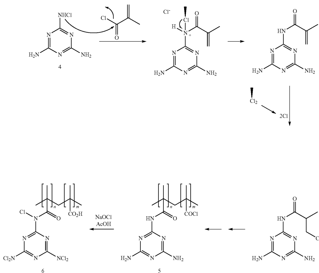
Scheme 3. Preparation of poly(melamine methacrylamide -co-methacryloyl chloride) and subsequent chlorination
