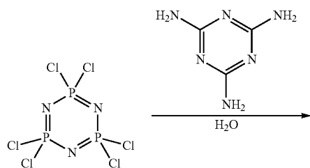
Scheme 11. Preparation of hexakis-melamine cyclotriphosphazene
