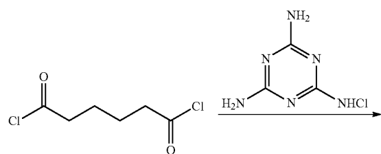
Scheme 7. Preparation of bismelamine adipoyl
