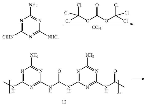
Scheme 6. Preparation of polyurea-melamines
