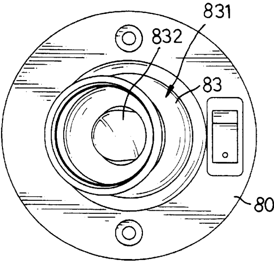
FIG. 9 PRIOR ART
