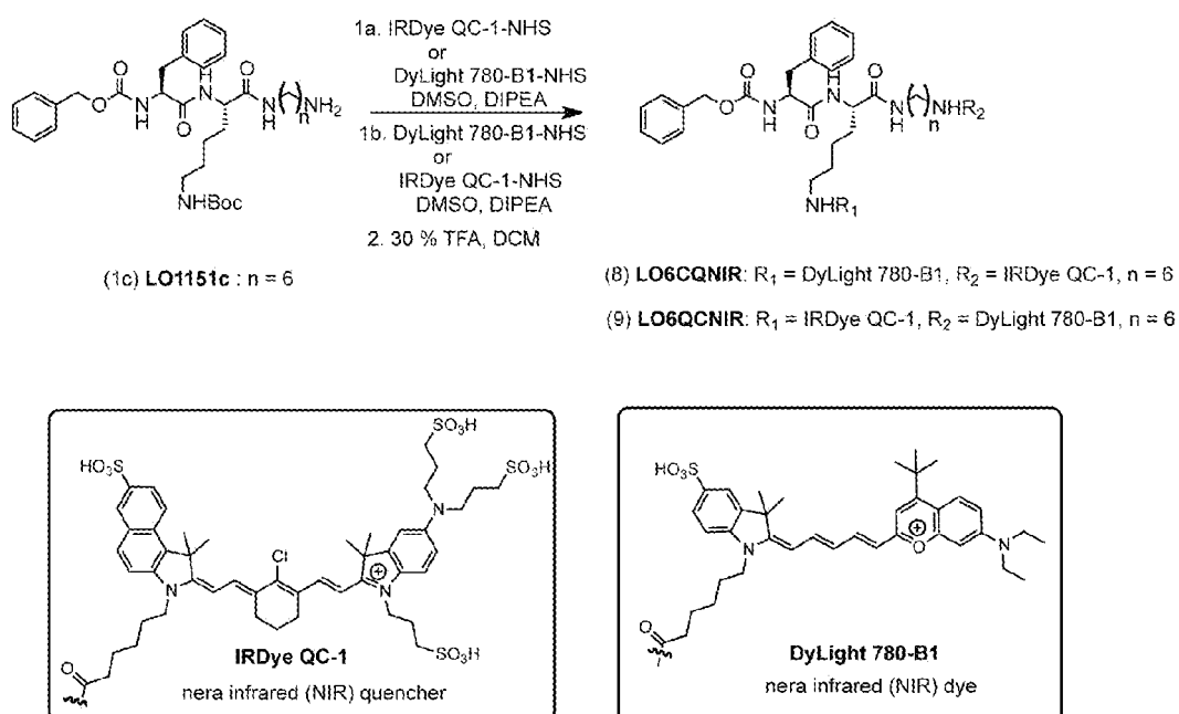
Scheme 2. Synthesis of near infrared non-covalent quenched fluorescent activity based probe compatible with the da Vinci surgical robot
