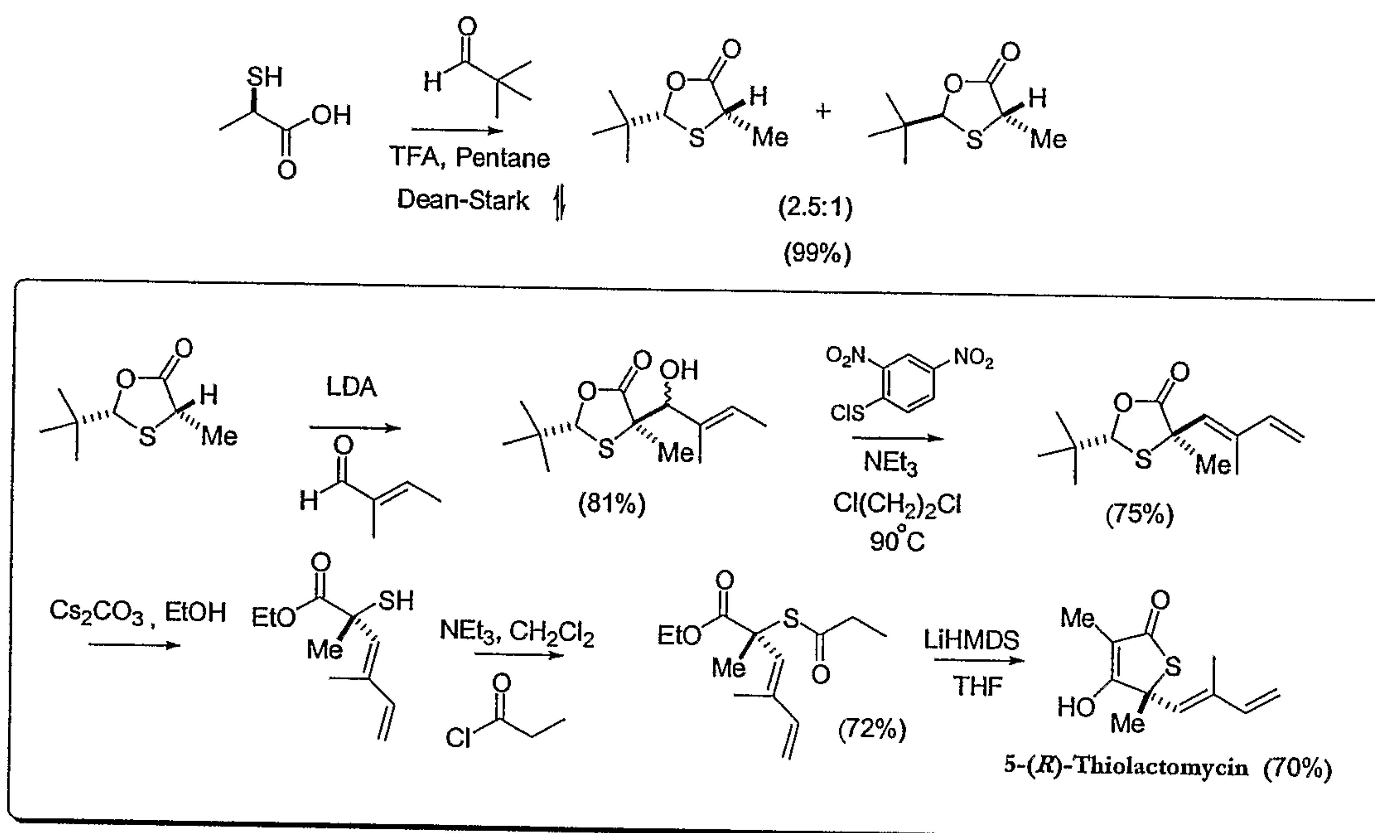
Scheme 1. Asymmetric Synthesis of 5-( R )-Thiolactomycin.
