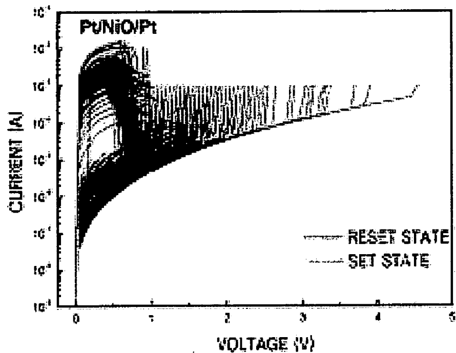
FIG. 5 (RELATED ART)
