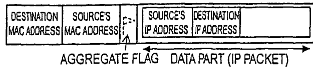
Fig. 20 20/20 FORMAT OF ETHERNET FRAME
