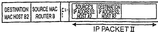
ETHERNET FRAME VII
