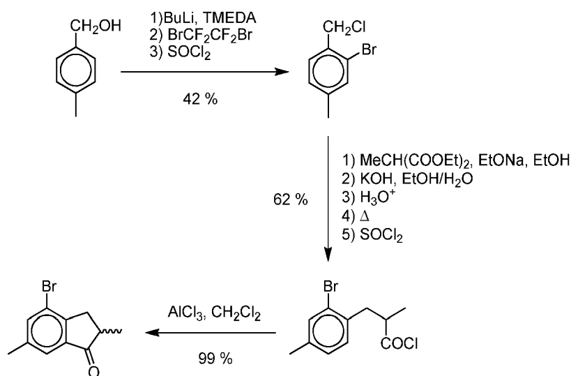
Scheme 2: synthesis of 2,6-dimethyl-4-bromoindanone
