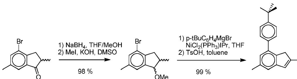
Scheme 3: synthesis of 2,6-dimethyl-4-(4'- tert -butylphenyl)indene
