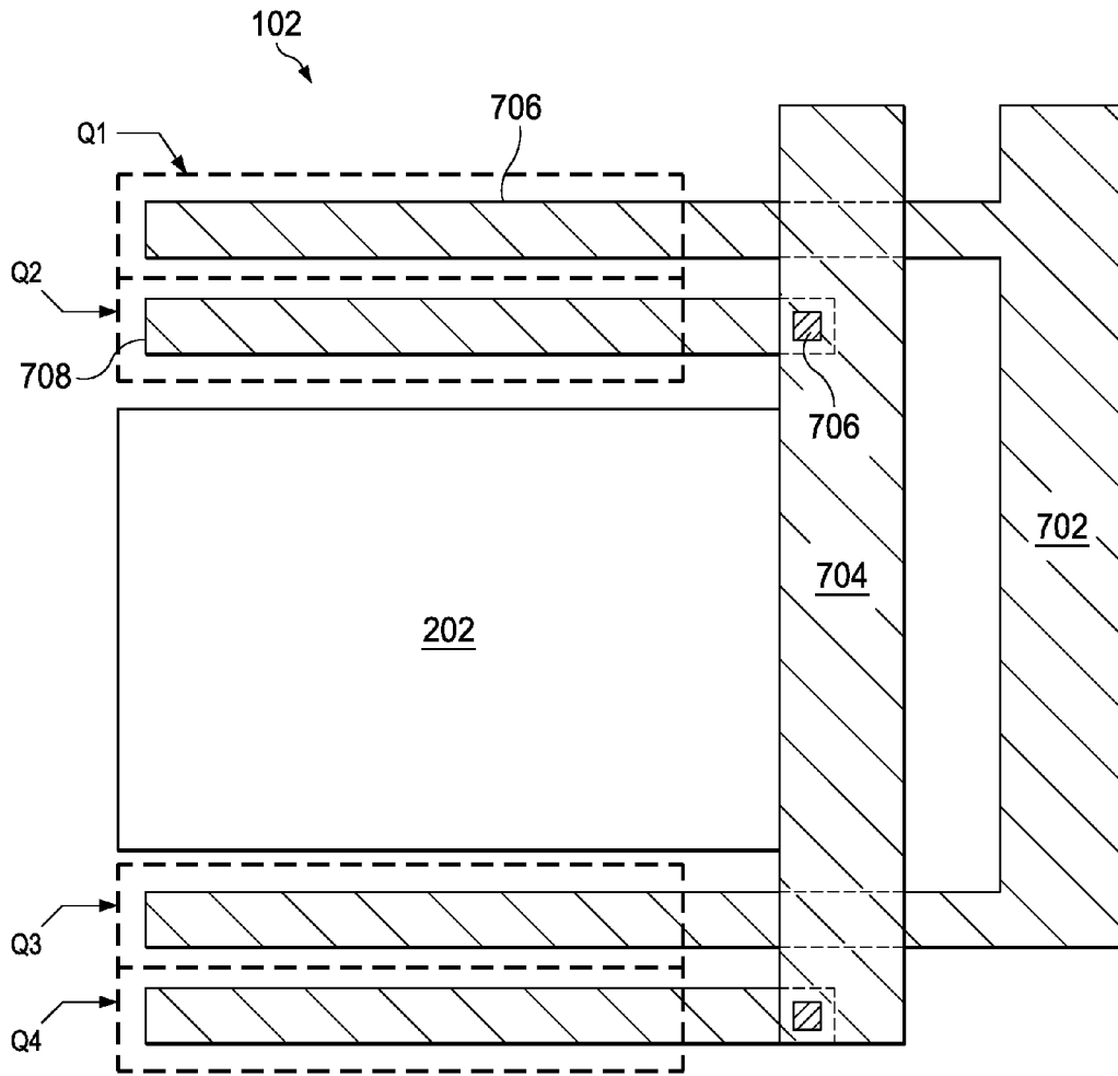
FIG. 7 (PRIOR ART)
