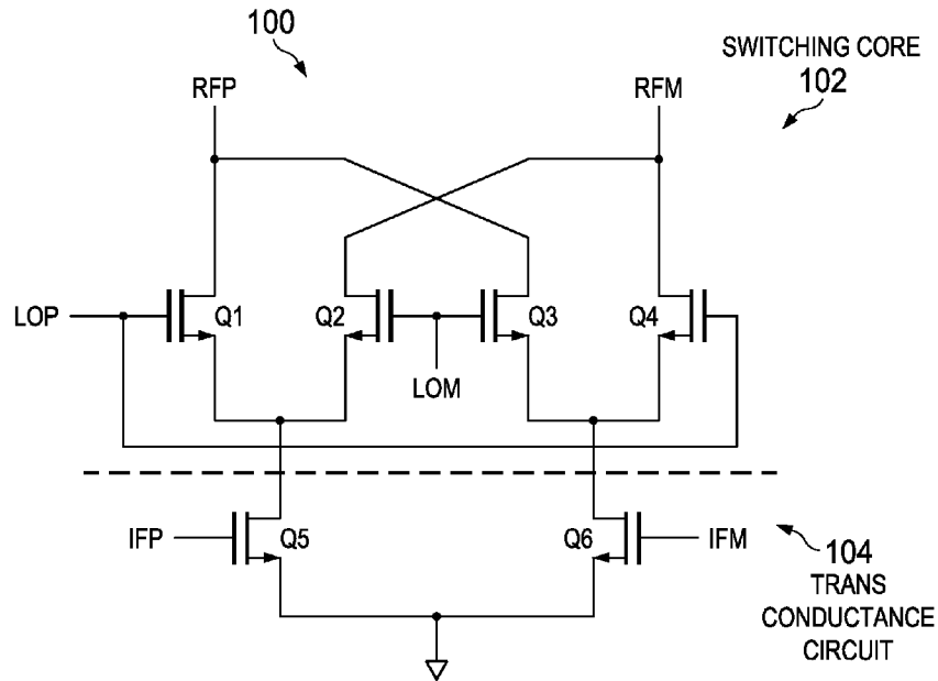
FIG. 1 (PRIOR ART)
