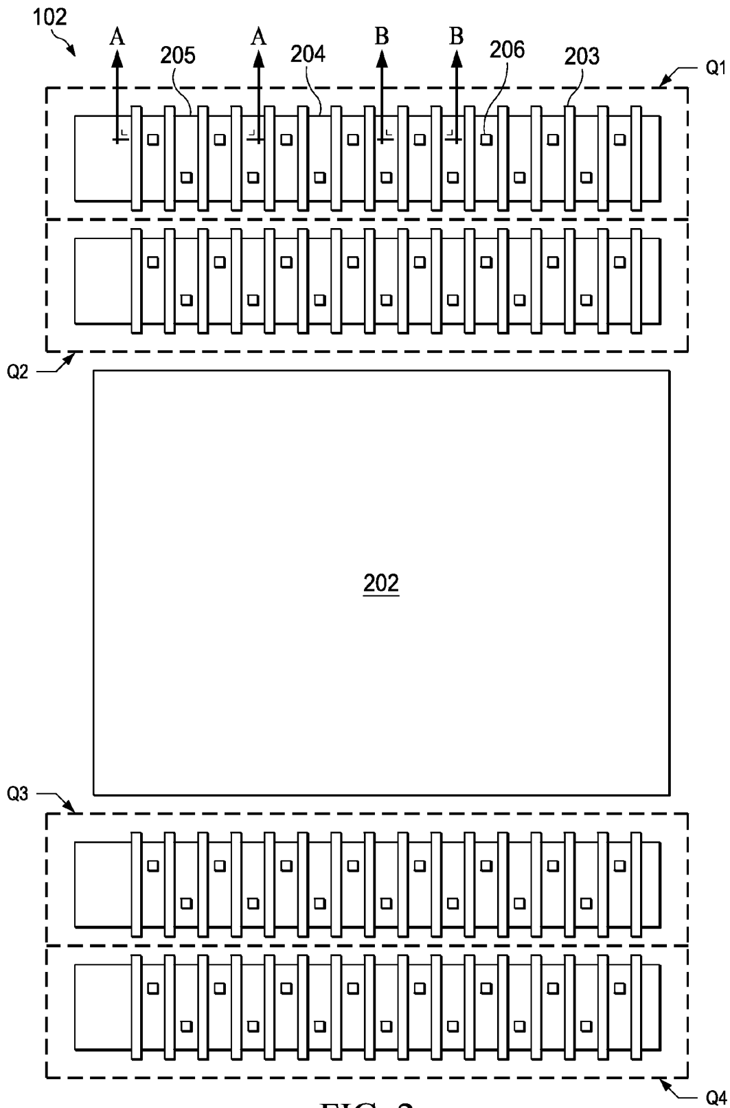
FIG. 2 (PRIOR ART)
