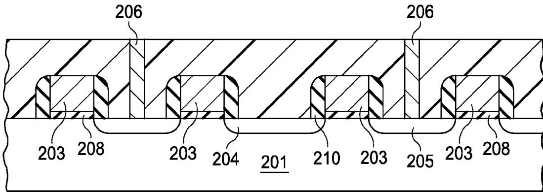
FIG. 3 (PRIOR ART)
