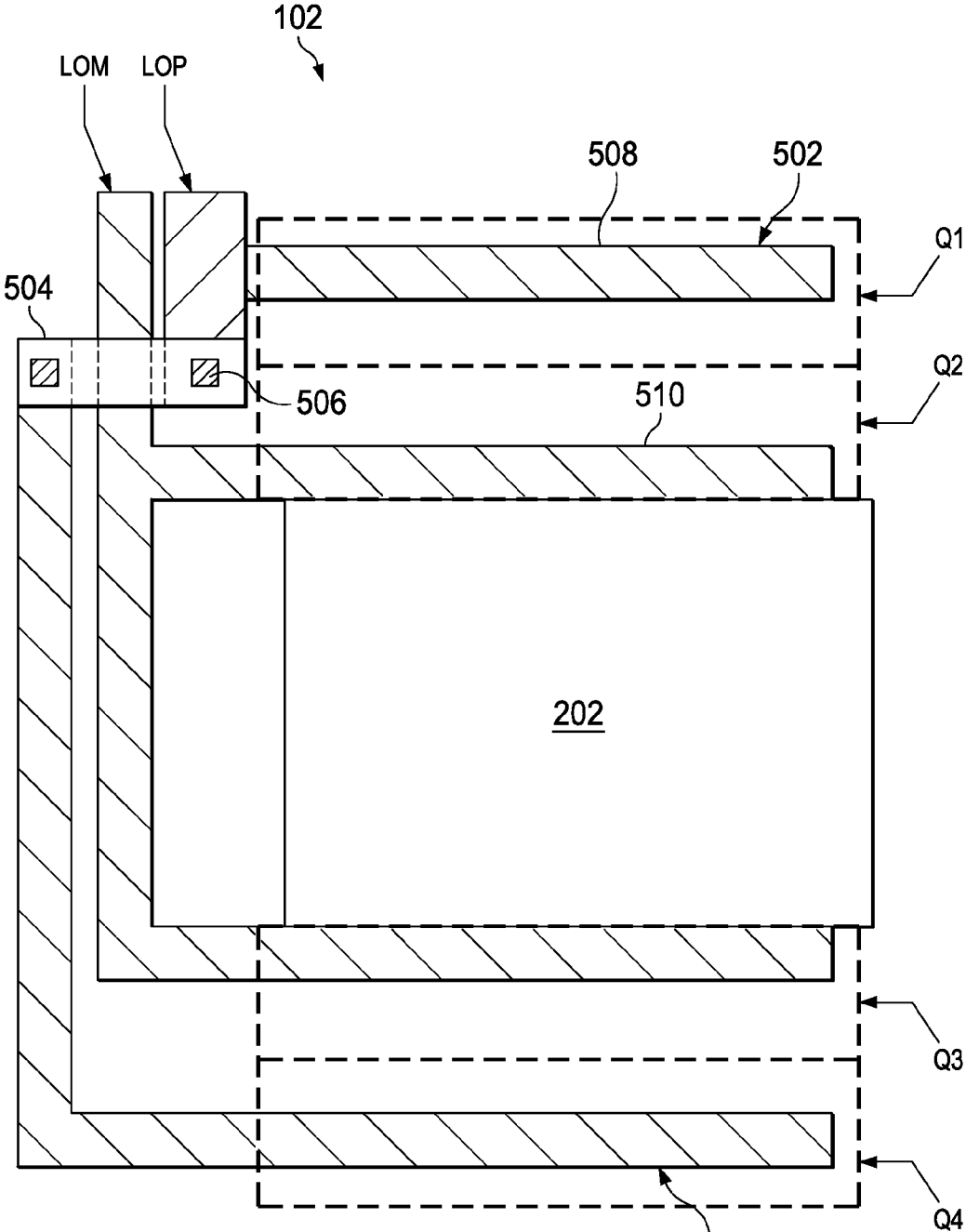
FIG. 5 (PRIOR ART)
