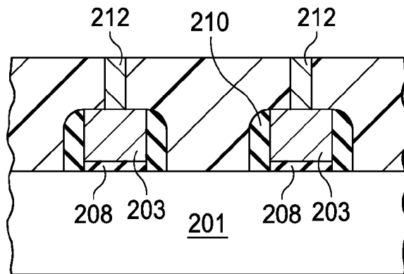
FIG. 4 (PRIOR ART)
