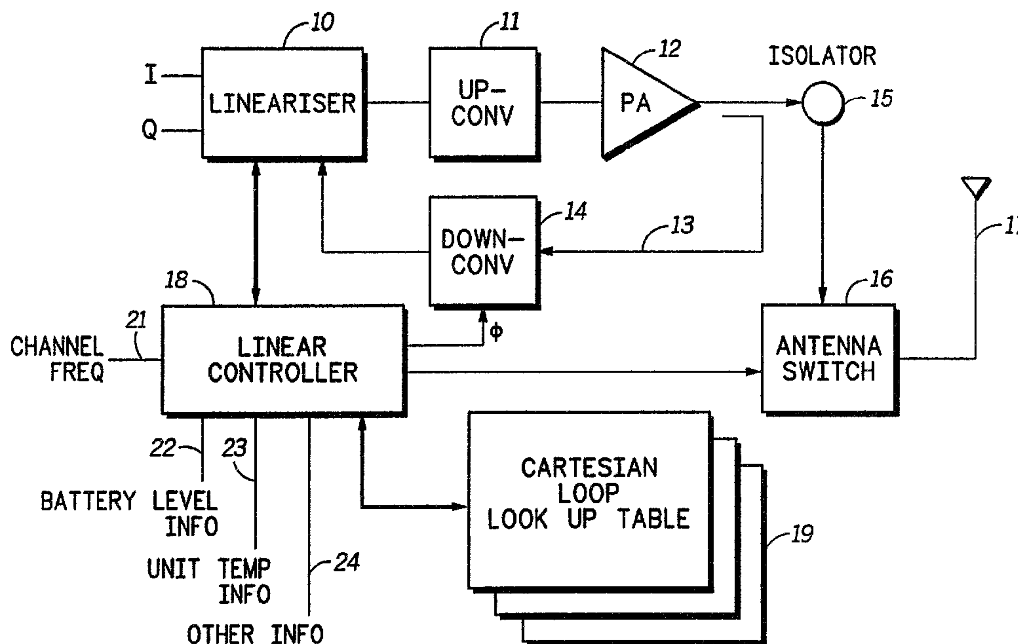
LINEARISER BLOCK DIAGRAM
