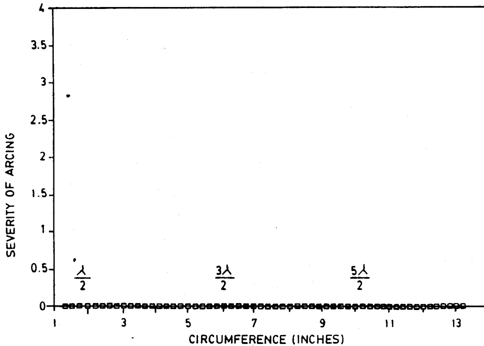
ARCING IN AN OVERLAPPED- FOIL LOOP
