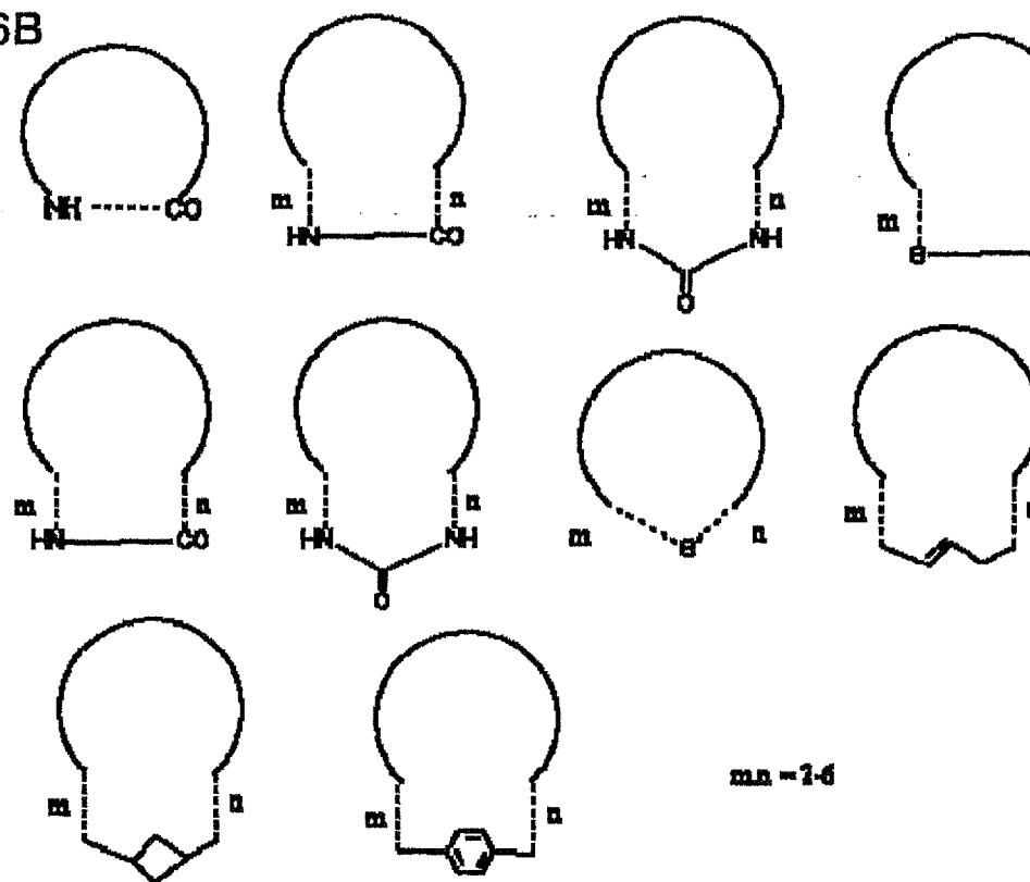
Scheme 2. Cyclization strategies:
