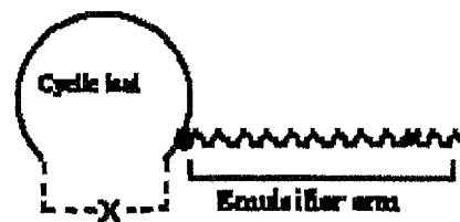
Scheme 1. General structure of the cyclic lead with amplifier arm
