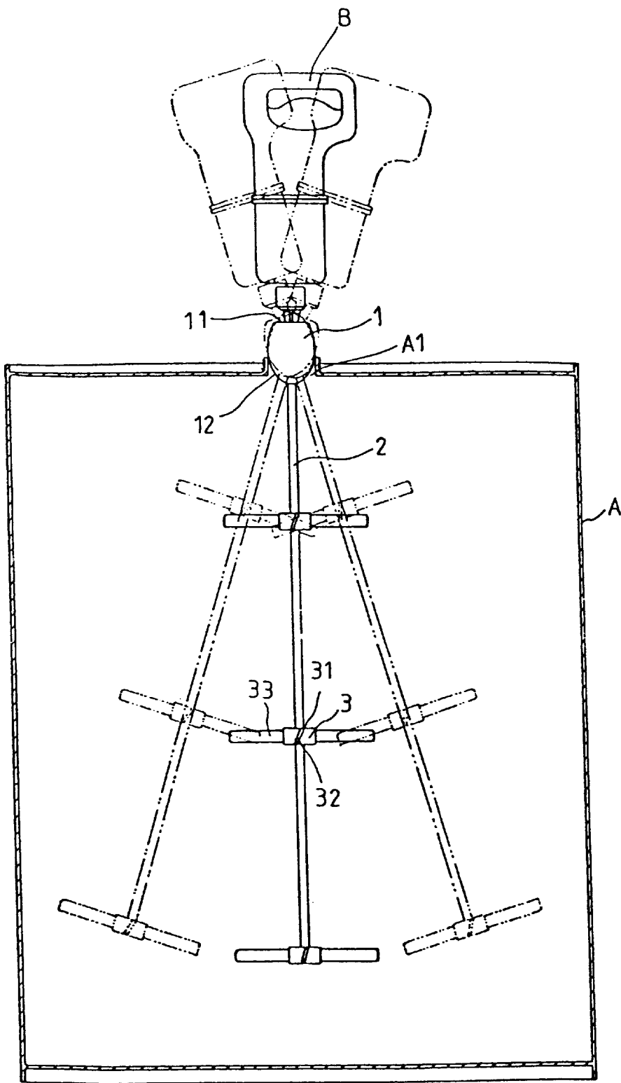
Fig. 1 PRIOR ART
