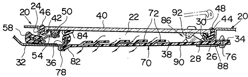
FIG. 2 PRIOR ART
