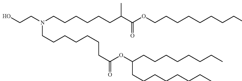
XX64. Compound 164: Nonyl 8-((8-(heptadecan-9-yloxy)-8-oxooctyl)(2-hydroxyethyl)amino)-2-methyloctanoate
