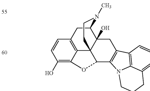
Registry number 189016-07-7
