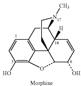
Chart 2. Opioid Receptor Ligands Morphine and Morphinans
