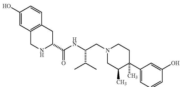
Registry number 361444-66-8
