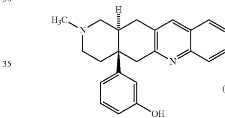
Registry number 189263-70-5
