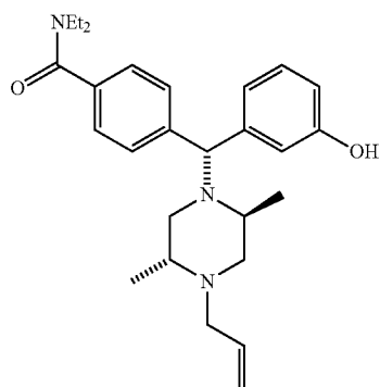
Registry Number 155836-52-5
