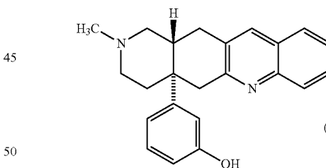
Registry number 173398-79-3
