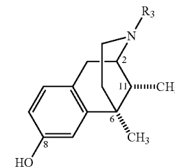
Chart 1. Opioid Receptor Ligands Benzomorphan (a.k.a. 2,6-Methano-3-benzazocines)
