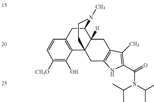
Registry number 177284-71-8
