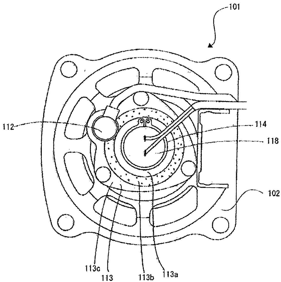
FIG. 2 PRIOR ART
