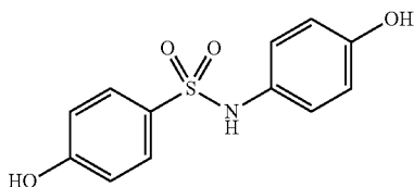
4-Hydroxy-N-(4-hydroxyphenyl)-benzenesulfonamide
