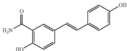
(E)-2-Hydroxy-5-(4-hydroxystyryl)benzamide
