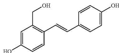
3-Hydroxymethyl-4-[(E)-2-(4-hydroxy-phenyl)-vinyl]-phenol
