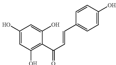
(E)-3-(4-Hydroxy-phenyl)-1-(2,4,6-trihydroxy-phenyl)-propenone
