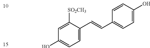
4-[(E)-2-(4-Hydroxyphenyl)vinyl]-3-methanesulfonylphenol
