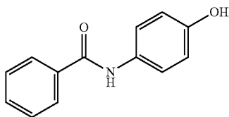
N-(4-Hydroxy-phenyl)-benzamide
