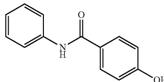
4-Hydroxy-N-phenyl-benzamide
