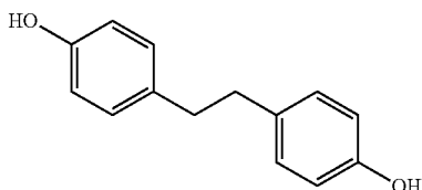
4-[4-Hydroxy-phenethyl]-phenol
