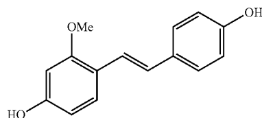
4-[(E)-2-(4-Hydroxyphenyl)-vinyl]-3-methoxy-phenol
