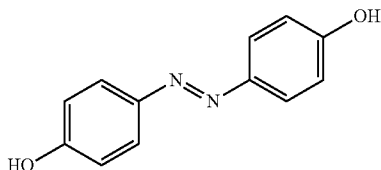
4-(4-Hydroxy-phenyl)-azophenol
