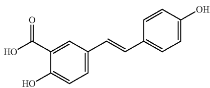
2-Hydroxy-5-[(E)-2-(4-hydroxyphenyl)vinyl]benzoic acid
