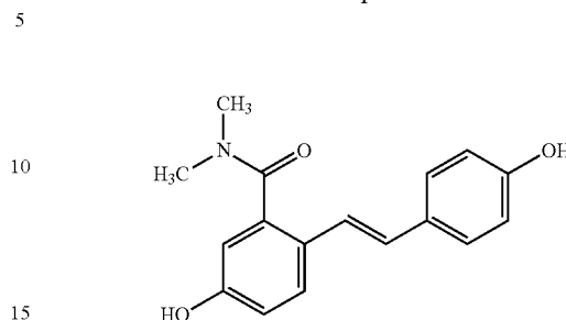
5-Hydroxy-2-[2-(4-hydroxyphenyl)vinyl]-N,N-dimethylbenzamide
