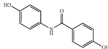
4-Hydroxy-N-(4-hydroxyphenyl)-benzamide
