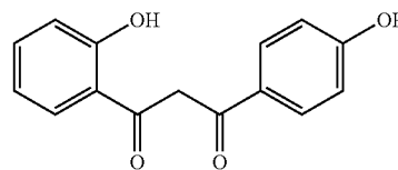
1-(4-Hydroxy-phenyl)-3-(2-hydroxy-phenyl)-propane-1,3-dione
