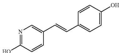
5-[(E)-2-(4-Hydroxyphenyl)-vinyl]-pyridin-2-ol
