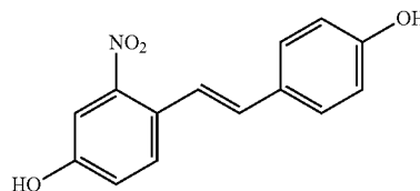
3-Nitro-4-[(E)-2-(4-hydroxyphenyl)-vinyl]phenol
