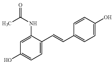
N-{5-Hydroxy-2-[(E)-2-(4-hydroxyphenyl)vinyl]phenyl}-acetamide
