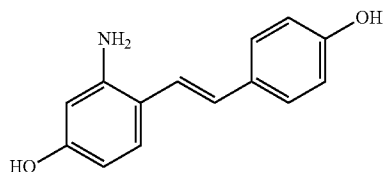
3-Amino-4-[(E)-2-(4-hydroxy-phenyl)vinyl]phenol
