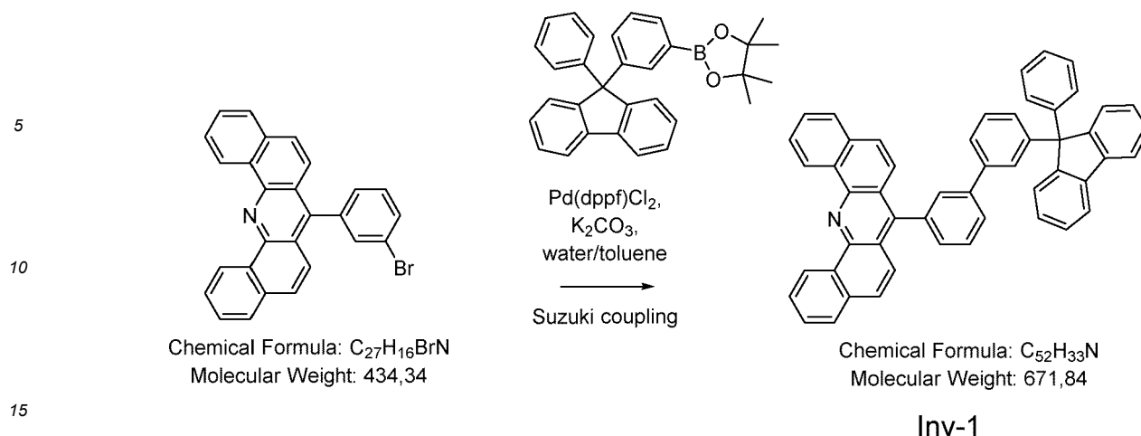
Scheme 1: Synthesis of 7-(3'-(9-phenyl-9H-fluoren-9-yl)-[1,1'-biphenyl]-3-yl) dibenzo [c,h]-acridine.
