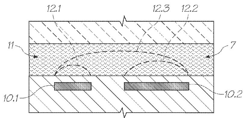
FIG. 52 (PRIOR ART)
