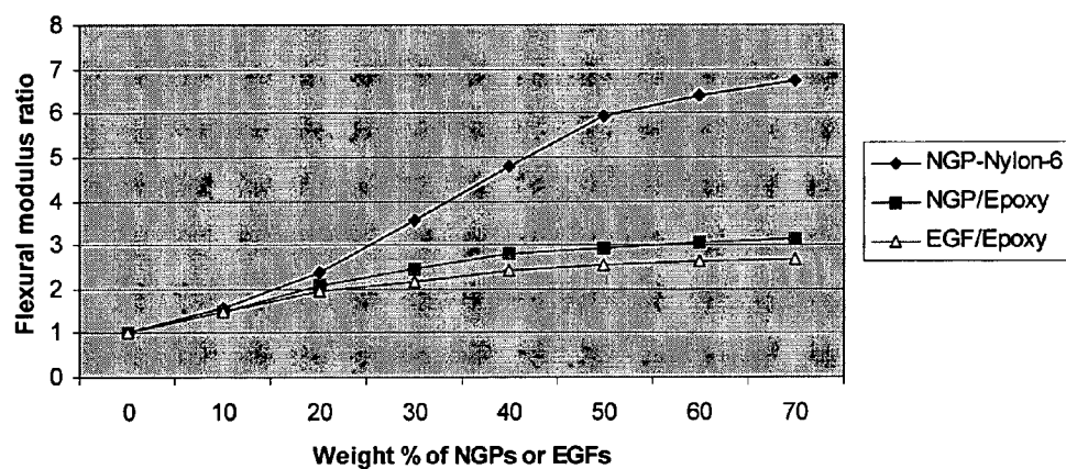
FIG.7(B) Composite-to-matrix modulus ratio.
