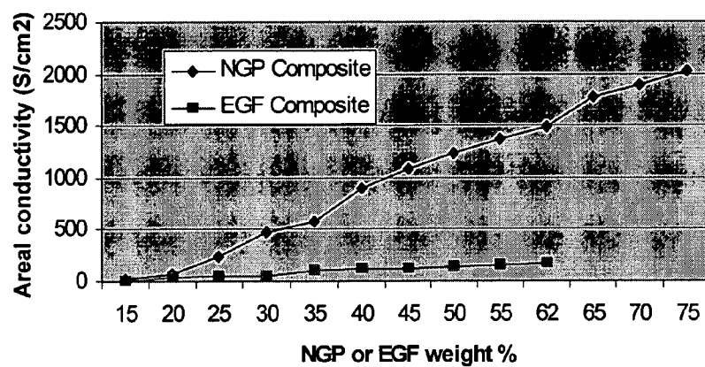
FIG.6 Areal conductivity of NGP- and EGF-polymer composites.
