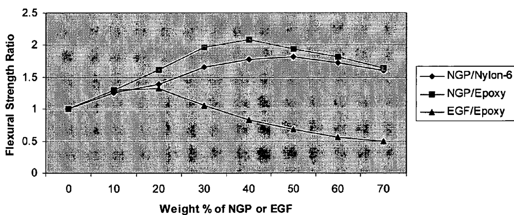
FIG.8(B) Ratio of composite strength to matrix strength.
