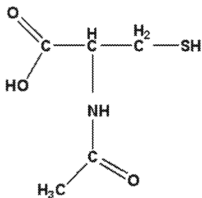
N-Acetylcysteine (NAC)
