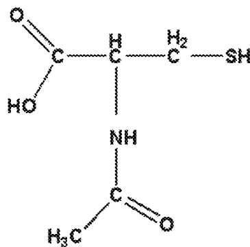
N-Acetylcysteine (NAC)
