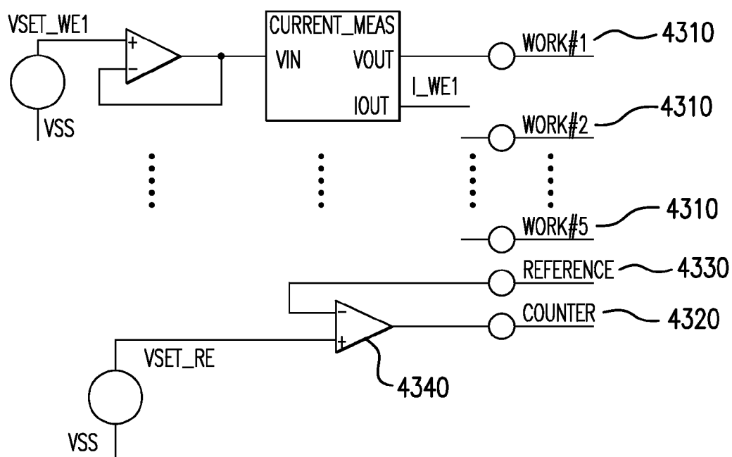
POTENTIOSTAT CONFIGURATION
