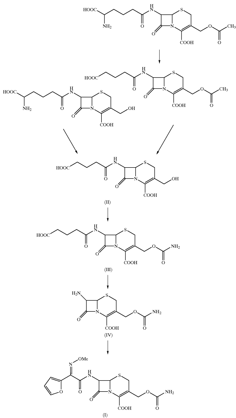
SCHEME 2
