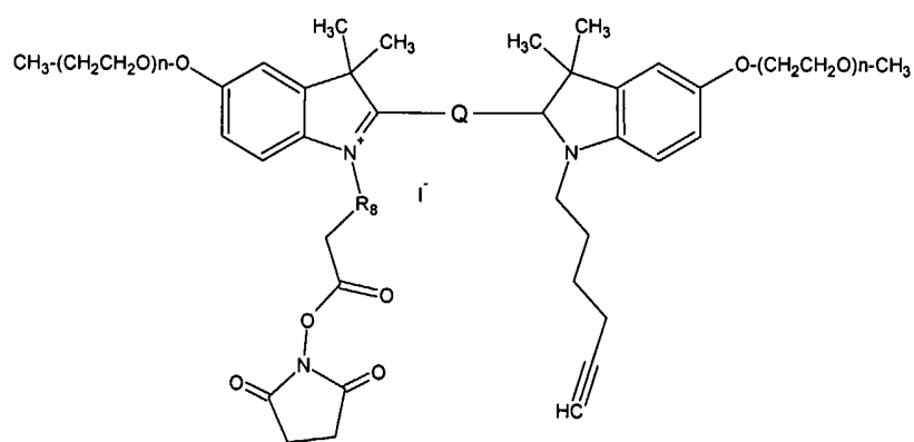
Formula (II)
