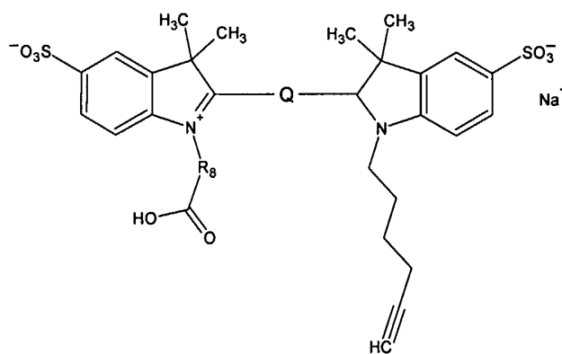
Formula (Ib)
