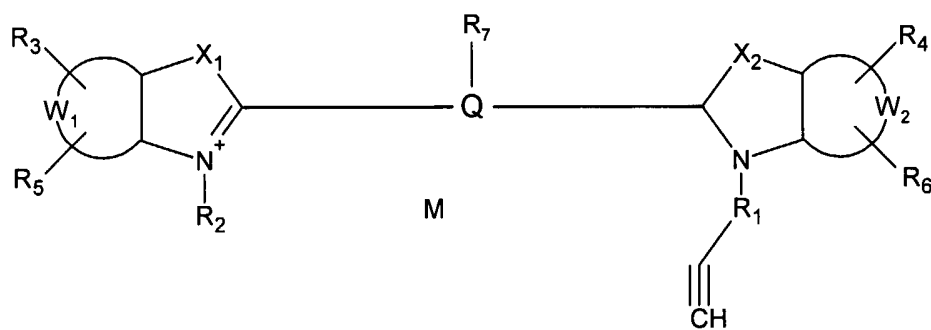
(I)
