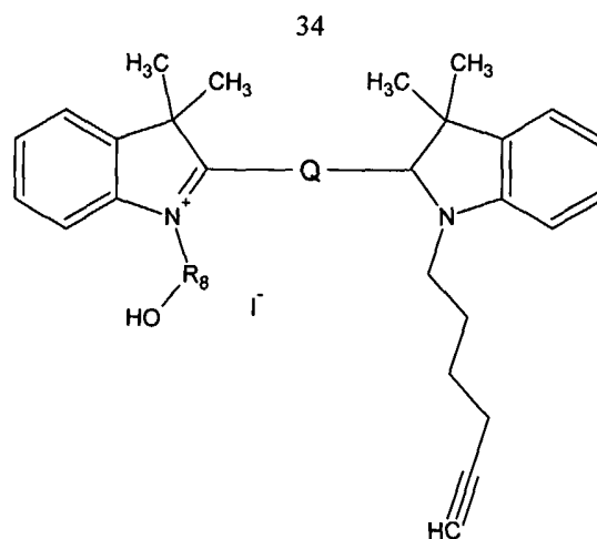
Formula (In),
