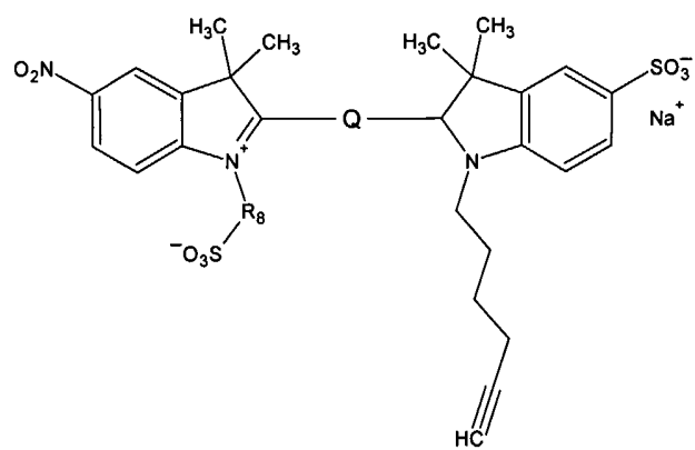
Formula (Ig)
