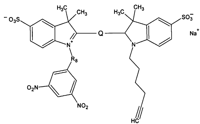
Formula (Id)
