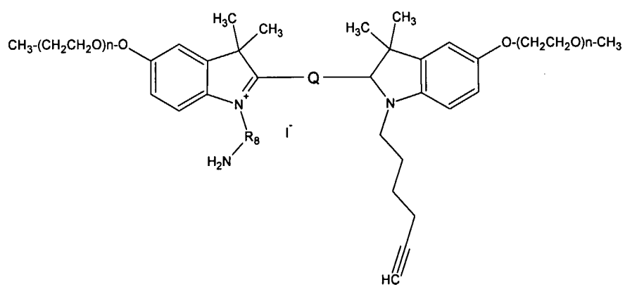
Formula (Im)
