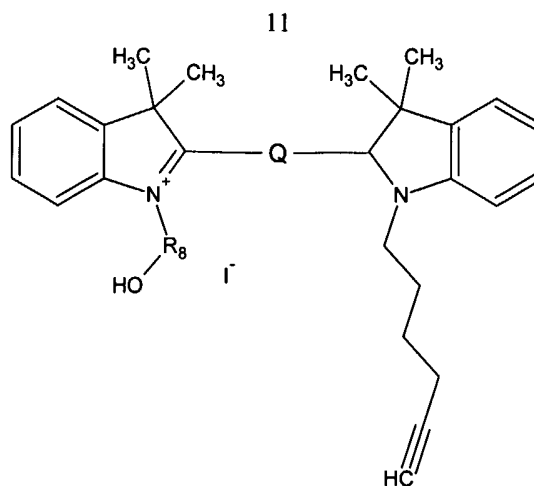
Formula (In)
