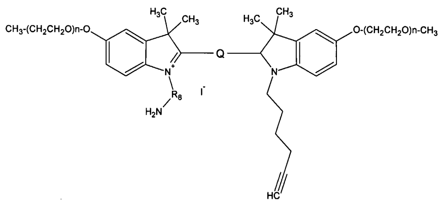
Formula (Im)
