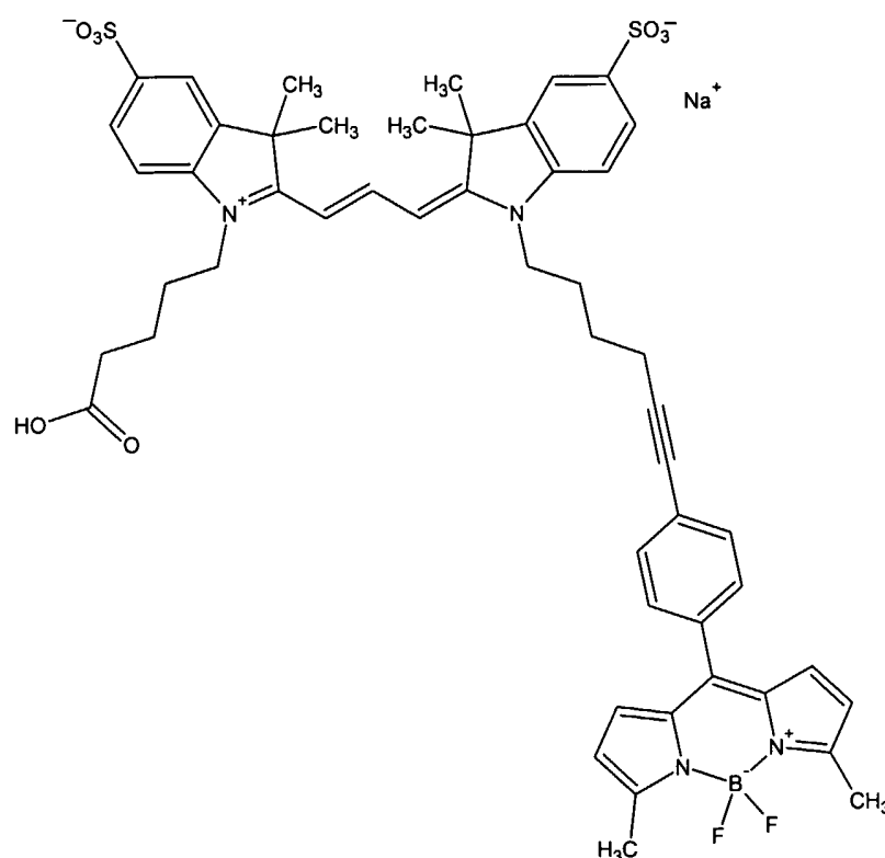
Formula (IIIa)
