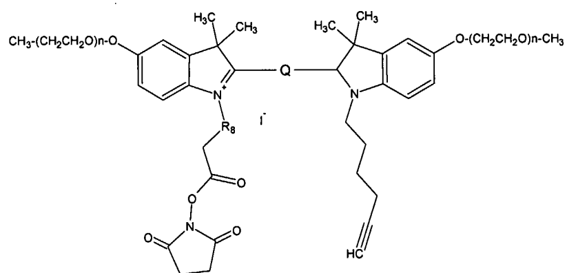
Formula (II)
