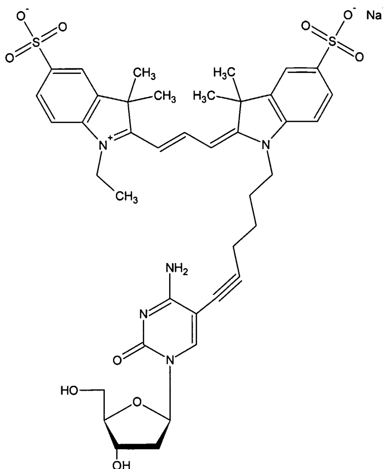
Compound 2
