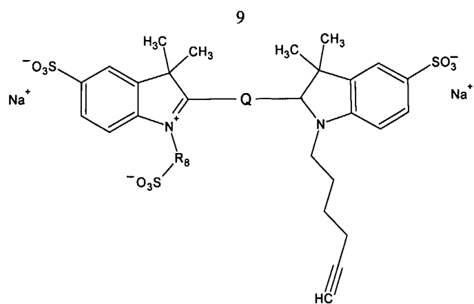
Formula (If)
