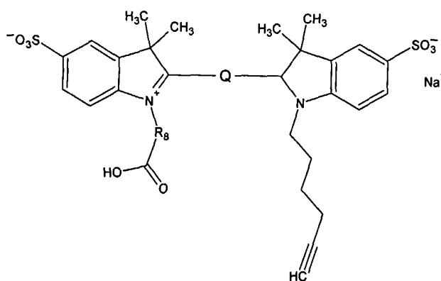
Formula (Ib)
