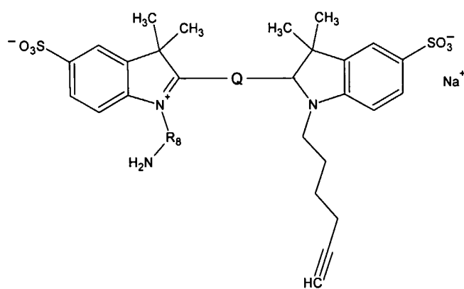
Formula (Ie)
