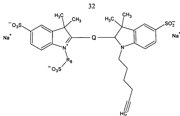
Formula (If)
