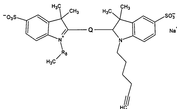
Formula (Ia)
