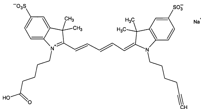
Compound 4
