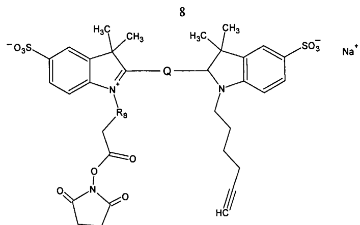
Formula (Ic)
