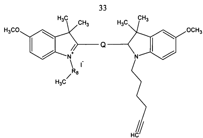
Formula (Ii)
