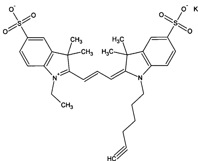
Compound 1
