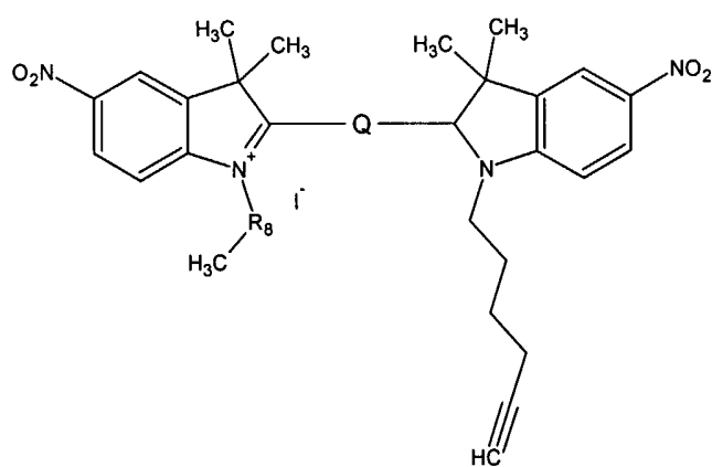
Formula (Ih)
