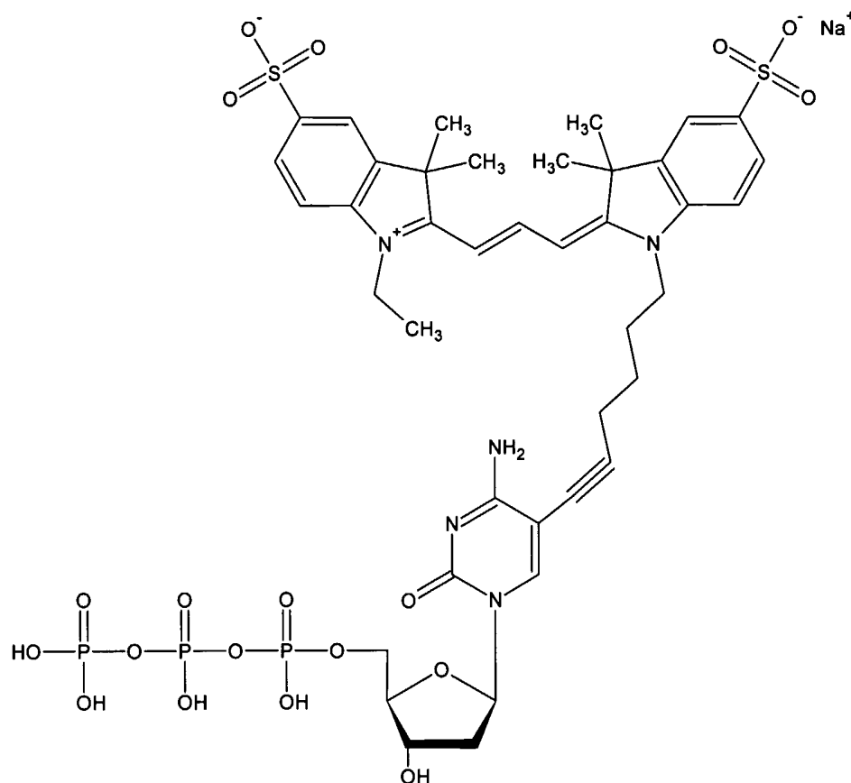
Compound 3
