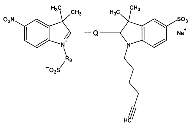
Formula (Ig)
