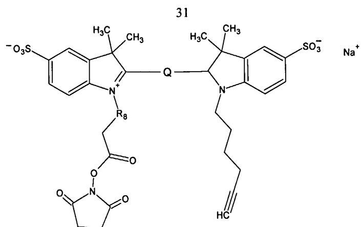
Formula (Ic)
