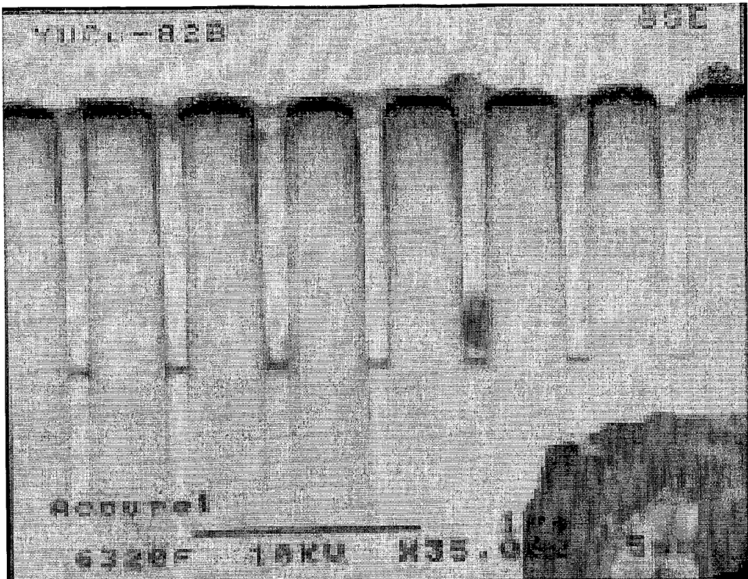
Figure 4 shows a reverse contrast cross-sectional micrograph of copper-filled 0.1 \times 1.0 \mu\text{m} trenches on TaN-coated silicon substrate.
