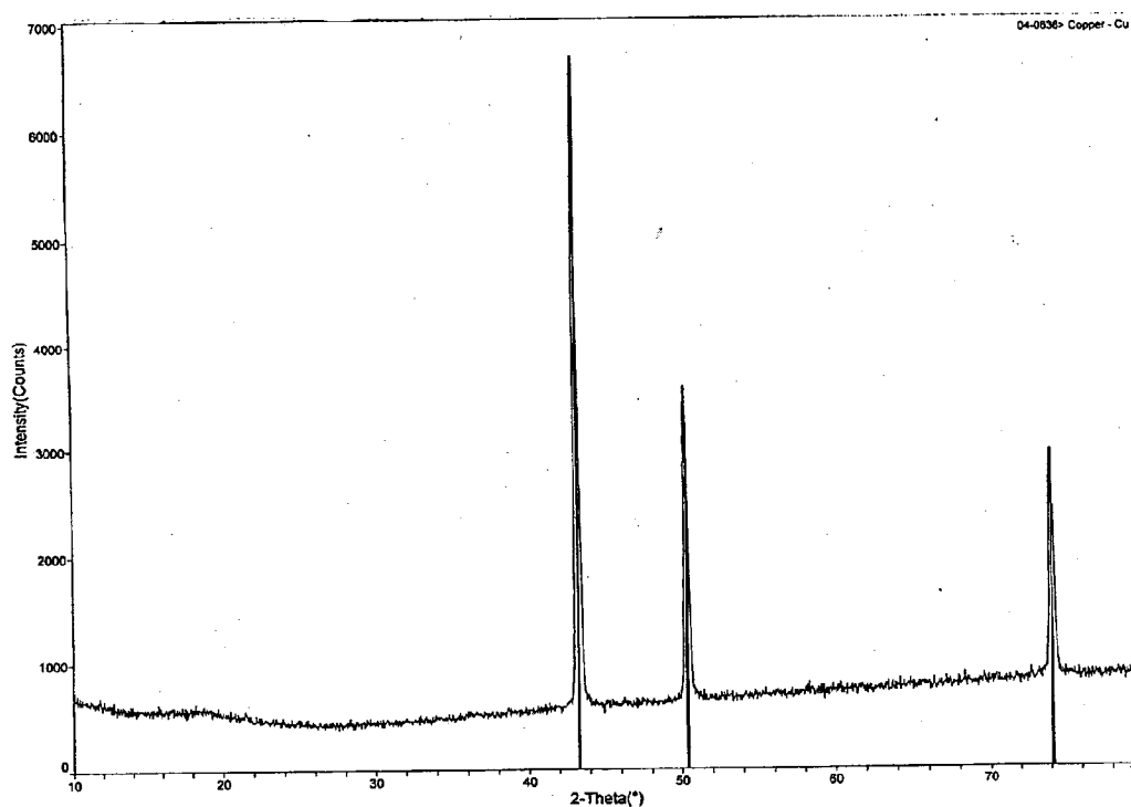
Figure 2 : X-Ray diffraction spectrum of copper nanocrystals after heating to 300 °C with reference copper metal spectrum overlaid.
