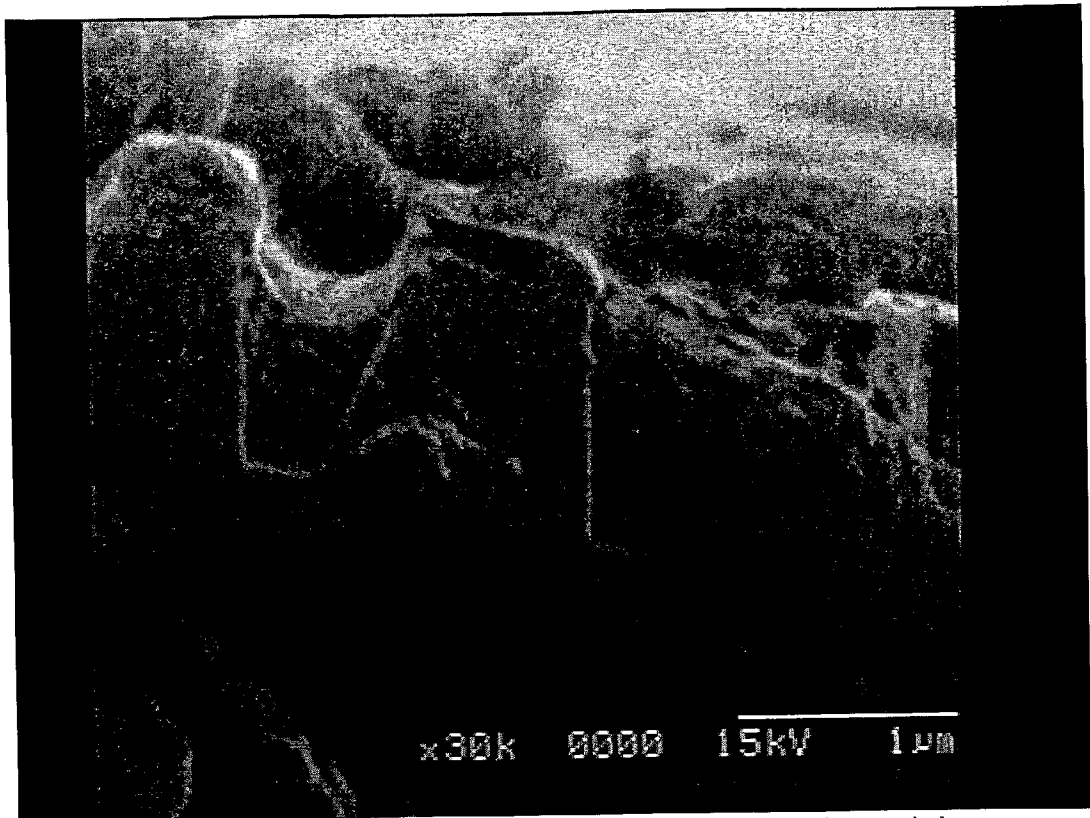
Figure 3 shows conformal, bottom-up fill of trenches with copper nanocrystals prior to heating.
