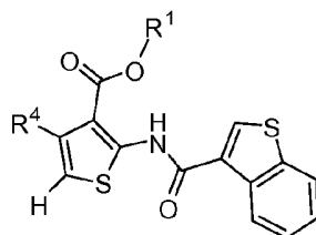
Formula (IIA)
