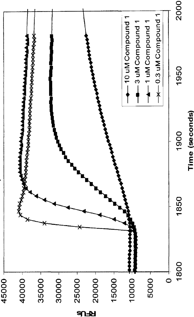
Figure 2. Effects of Compound 1 on the Kinetics of the CRAC Channel Response in RBL-2H3 Cells
