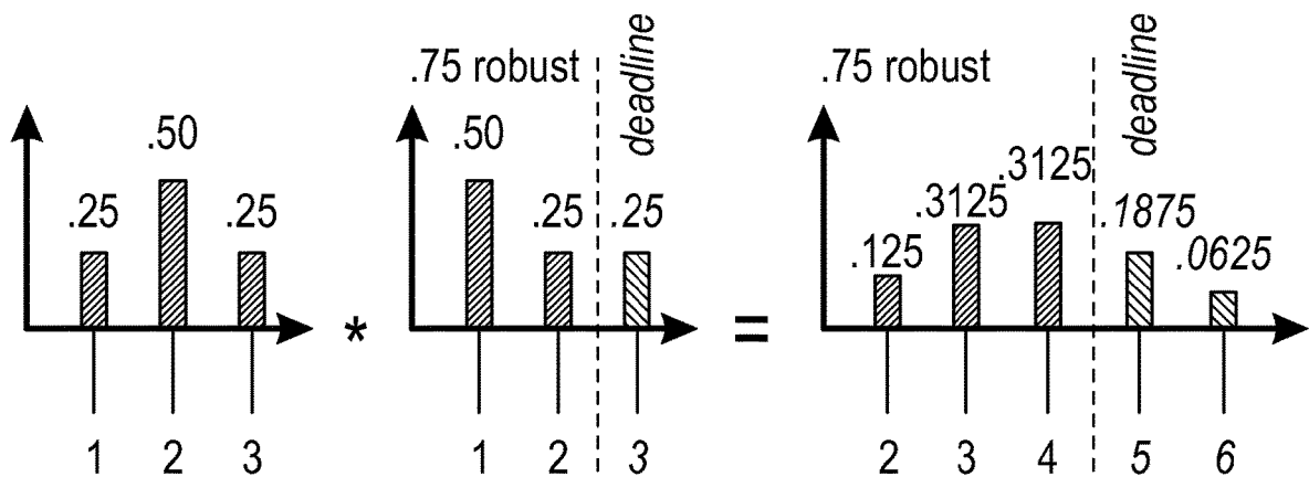
(c) Right Skew
