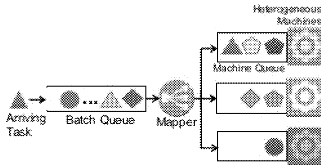
(b) Batch-mode resource allocation.
