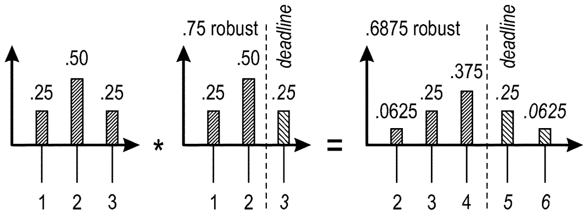
(a) No Skew
