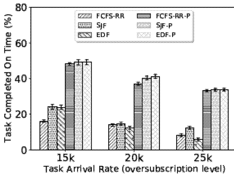
(b) Spiky Arrival Pattern
