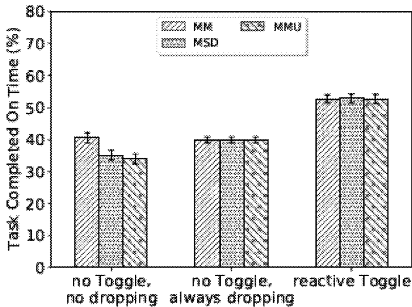
(b) Batch-mode mapping heuristics
