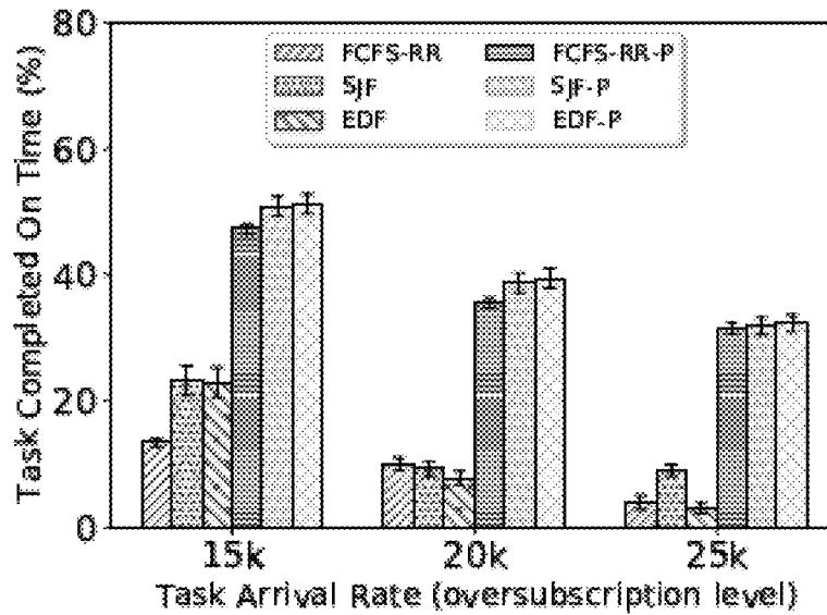
(a) Constant Arrival Pattern
