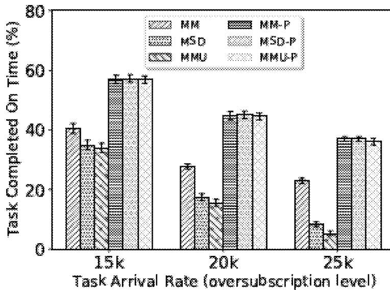
(b) Spiky Arrival Pattern
