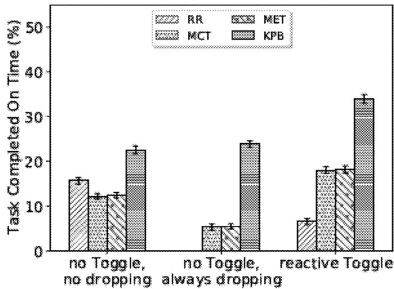
(a) Immediate-mode mapping heuristics
