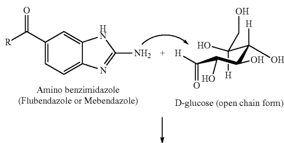
[Reaction Scheme 2]
