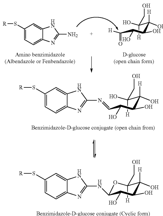
[Reaction Scheme 1]
