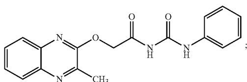
1-[2-(3-Methyl-quinoxalin-2-yloxy)-acetyl]-3-phenyl-urea (3x)
