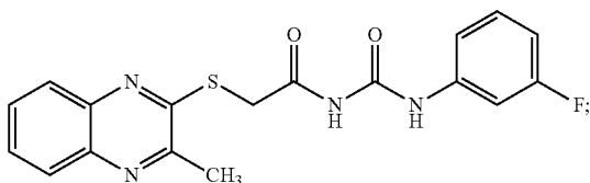
N-((4-fluorophenyl)carbamoyl)-2-((3-methylquinoxalin-2-yl)thio)acetamide (3w)
