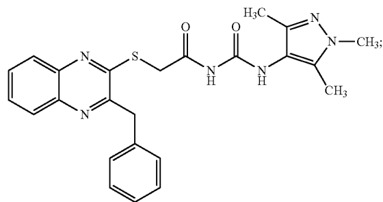
2-((3-benzylquinoxalin-2-yl)thio)-N-((1,3,5-trimethyl-1H-pyrazol-4-yl)carbamoyl)acetamide (3ac)
