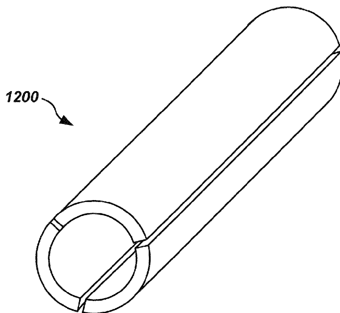
FIG. 11 Another Example Multi-Sectional Core Embodiment
