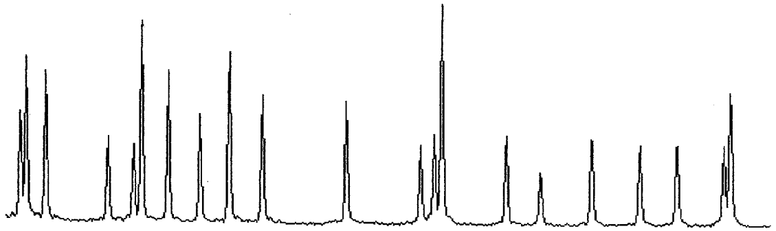
6-FAM-ddCTP 250 pm
