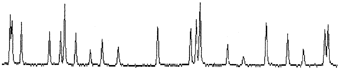
6-FAM-EO-ddCTP 50 pm
