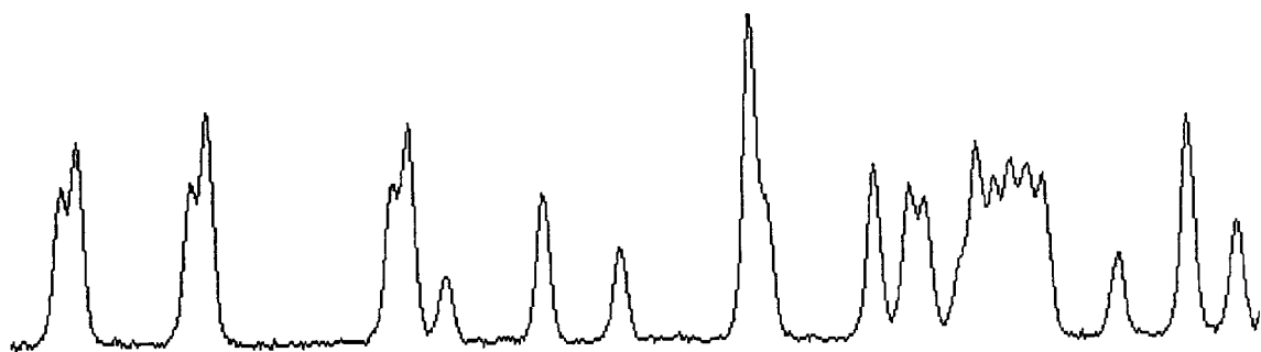
DTAMRA-1-labeled ddCTP using a propargylamido linker
