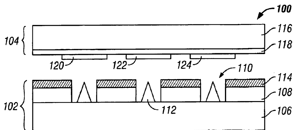
FIG. 1 (Prior Art)
