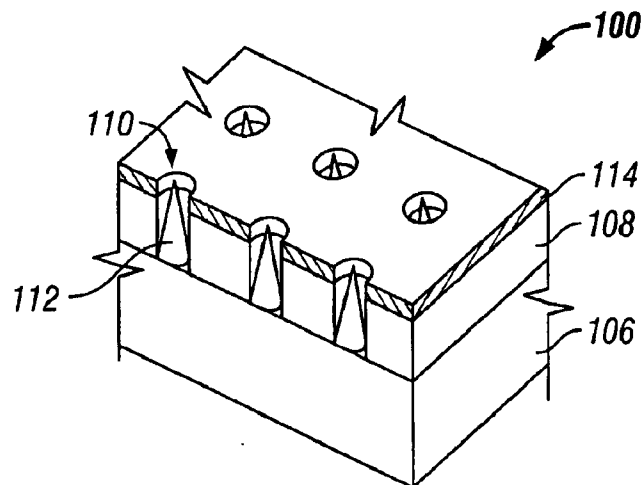
FIG. 3 (Prior Art)
