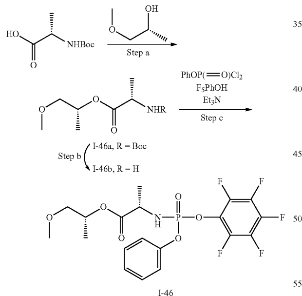
Step a) (S)—(R)-1-Methoxypropan-2-yl 2-(((tert-butoxycarbonyl)amino)propanoate (I-46a)
