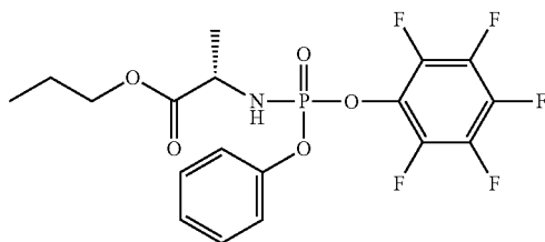
(2S)-Propyl 2-(((perfluorophenoxy)(phenoxy)phosphoryl)amino)propanoate (I-42)
