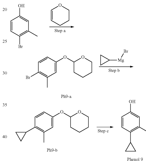
Step a) 2-(4-Bromo-3-methylphenoxy)tetrahydro-2H-pyran (Ph9-a)
