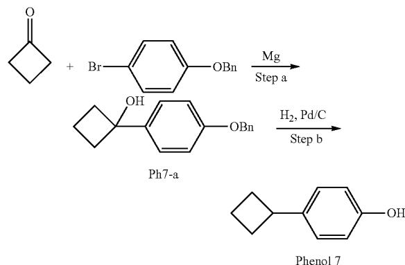
Step a) 1-(4-(benzyloxy)phenyl)cyclobutanol (Ph7-a)
