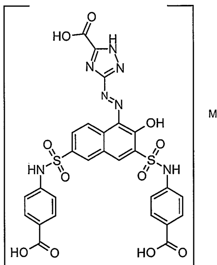
Compound (1)
