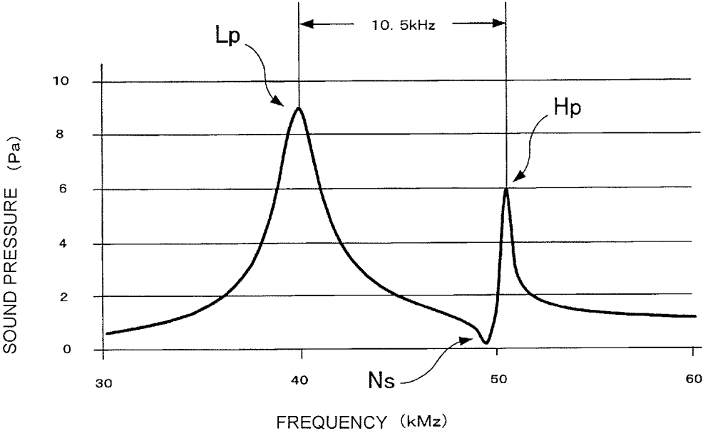
FREQUENCY-SOUND PRESSURE CHARACTERISTICS
