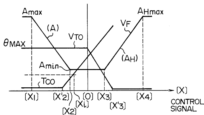
FIG. 6 PRIOR ART
