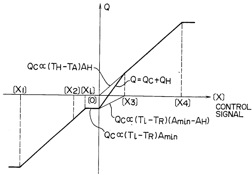
FIG. 7 (PRIOR ART)
